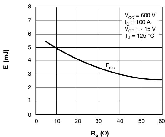
Fig. 9 - Diode Switching Loss vs. Gate Resistance
