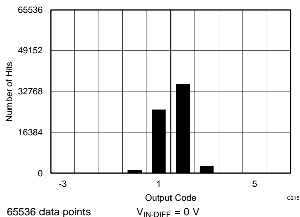
Figure 13. DC Histogram
