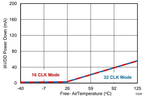
Figure 81. Power-Down Current vs Temperature
