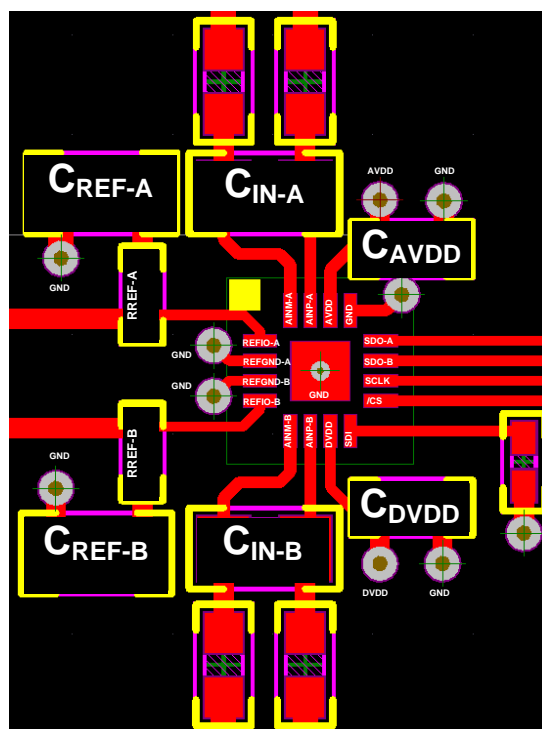
Figure 116. Recommended Layout
