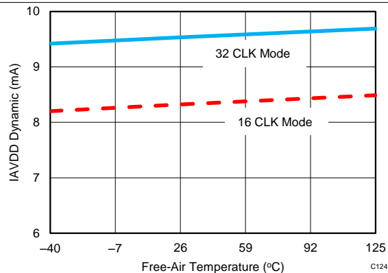
Figure 65. Analog Supply Current vs Temperature
