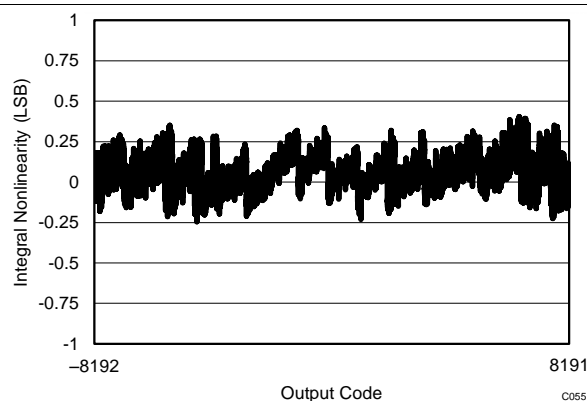
Figure 45. Typical INL
