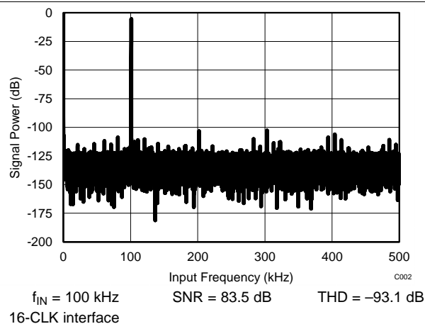
Figure 25. Typical FFT
