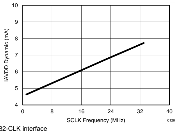
Figure 67. Analog Supply Current vs SCLK Frequency
