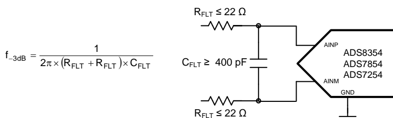
Figure 99. Antialiasing Filter
