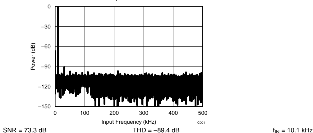
Figure 105. ADS7254 in 32-CLK Interface Mode
