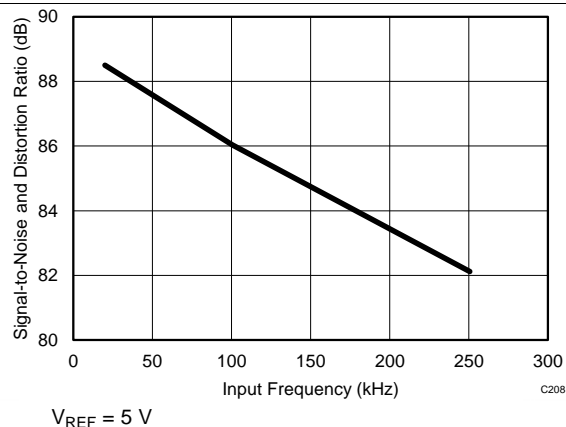
Figure 9. SINAD vs Input Frequency
