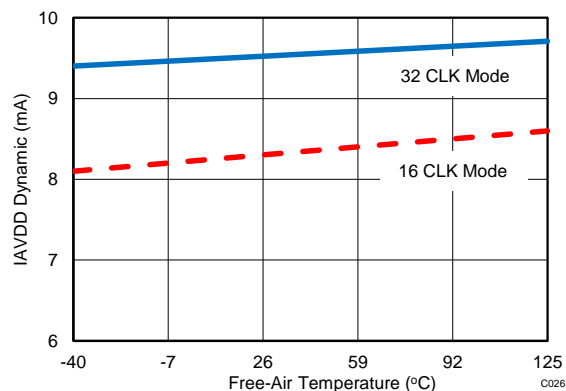
Figure 37. Analog Supply Current vs Temperature
