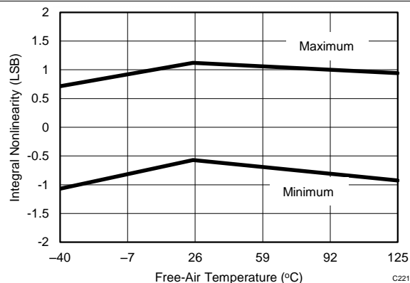
Figure 21. INL vs Temperature
