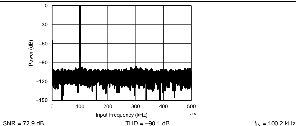
Figure 112. ADS7254 in 32-CLK Interface Mode
