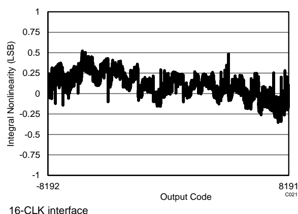
Figure 45. Typical INL
