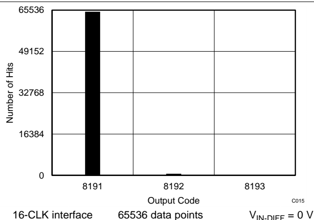
Figure 40. DC Histogram
