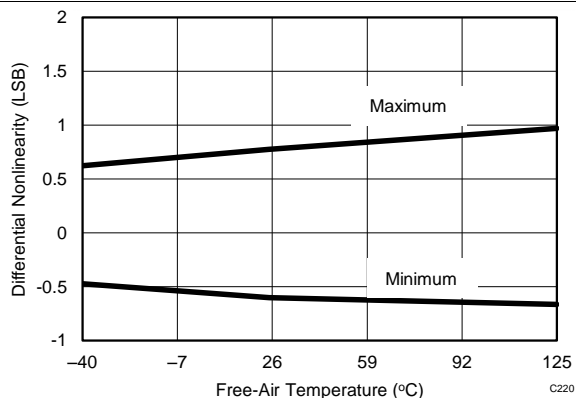
Figure 20. DNL vs Temperature
