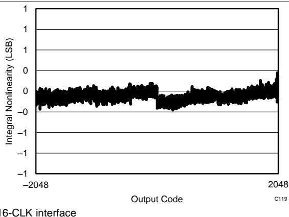
Figure 73. Typical INL
