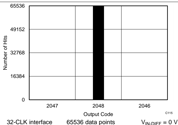
Figure 69. DC Histogram
