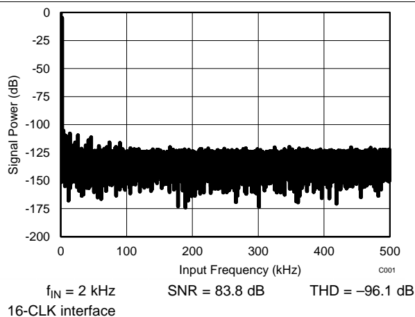
Figure 24. Typical FFT
