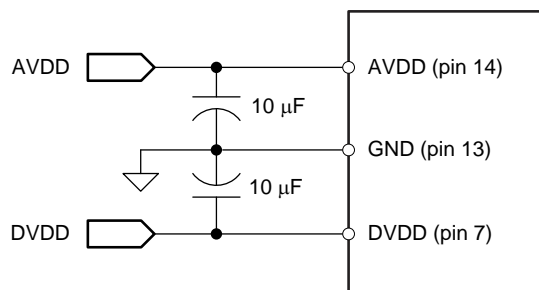
Figure 115. Power-Supply Decoupling
