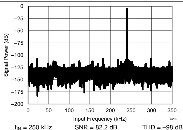
Figure 3. Typical FFT
