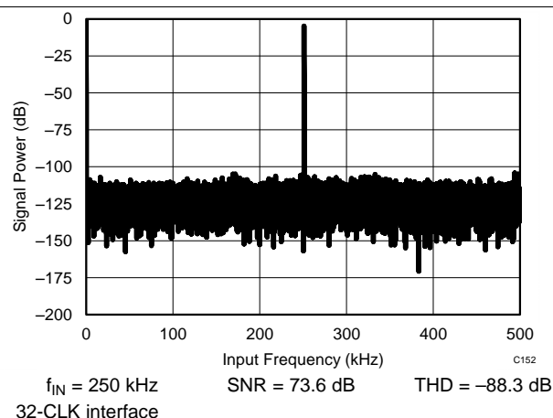
Figure 55. Typical FFT
