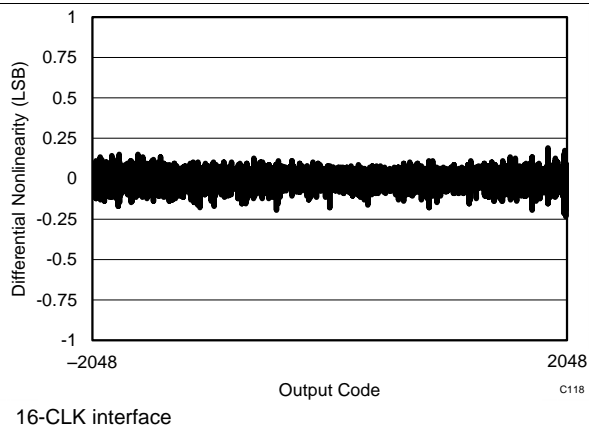
Figure 72. Typical DNL
