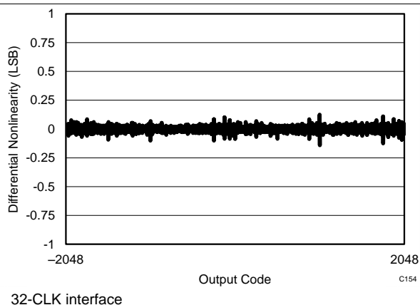
Figure 74. Typical DNL
