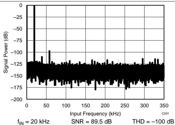
Figure 2. Typical FFT
