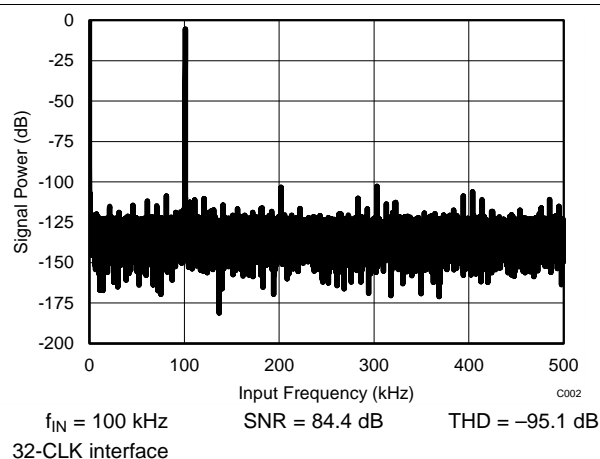
Figure 27. Typical FFT
