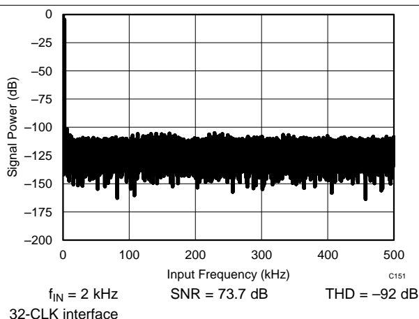
Figure 54. Typical FFT
