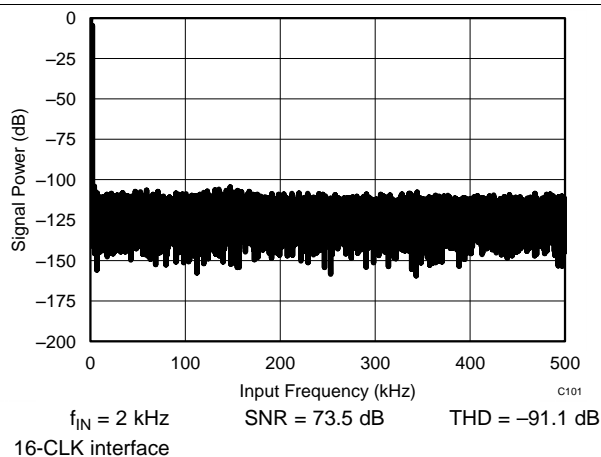
Figure 52. Typical FFT
