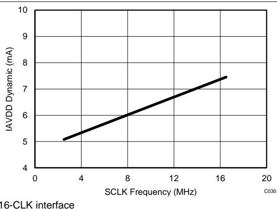
Figure 66. Analog Supply Current vs SCLK Frequency
