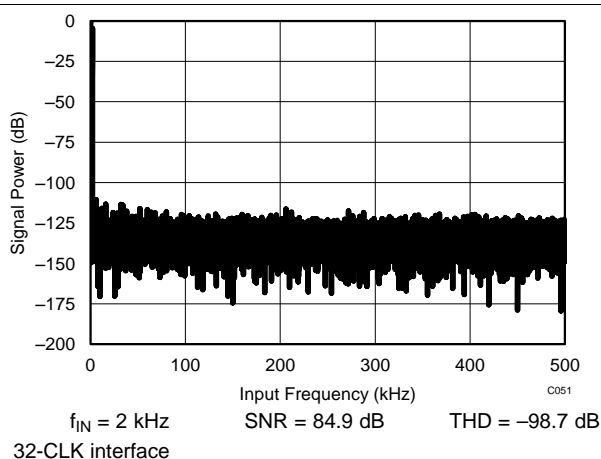
Figure 26. Typical FFT
