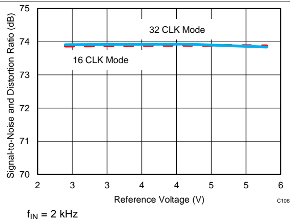
Figure 59. SINAD vs Reference Voltage
