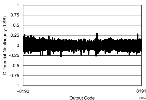
Figure 44. Typical DNL
