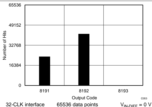
Figure 41. DC Histogram
