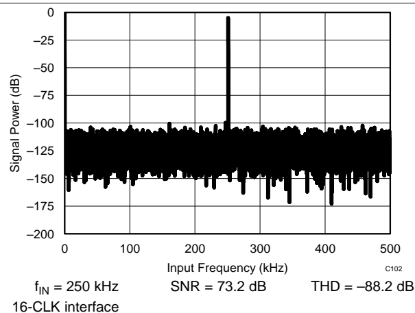
Figure 53. Typical FFT
