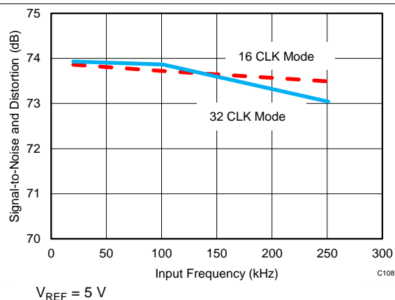
Figure 61. SINAD vs Input Frequency
