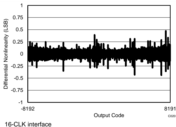
Figure 44. Typical DNL
