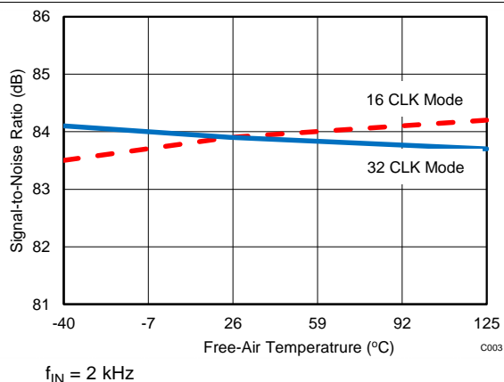
Figure 28. SNR vs Temperature
