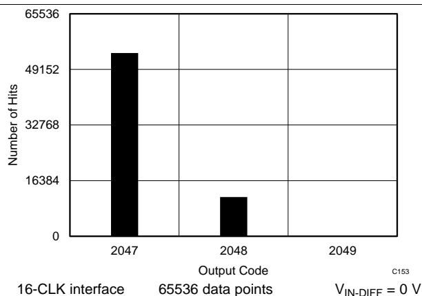
Figure 68. DC Histogram
