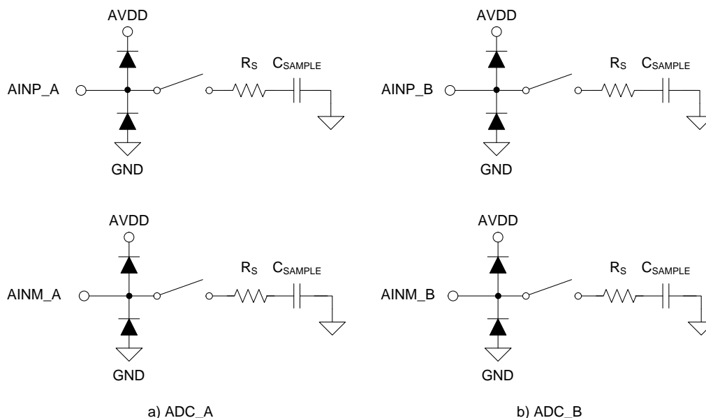
Figure 85. Equivalent Circuit for the Analog Input Pins
