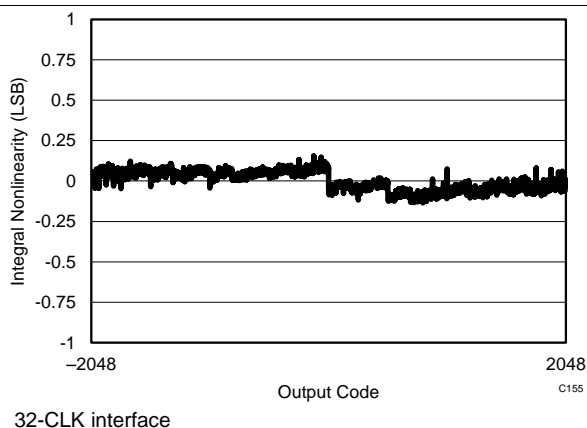
Figure 75. Typical INL
