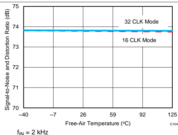
Figure 57. SINAD vs Temperature
