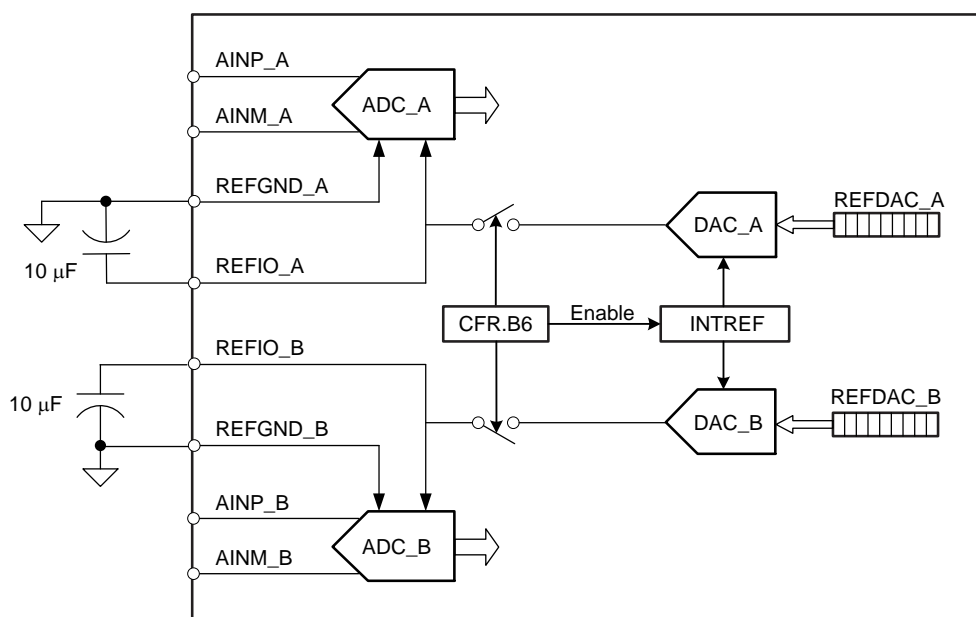
Figure 84. Reference Configurations and Connections
