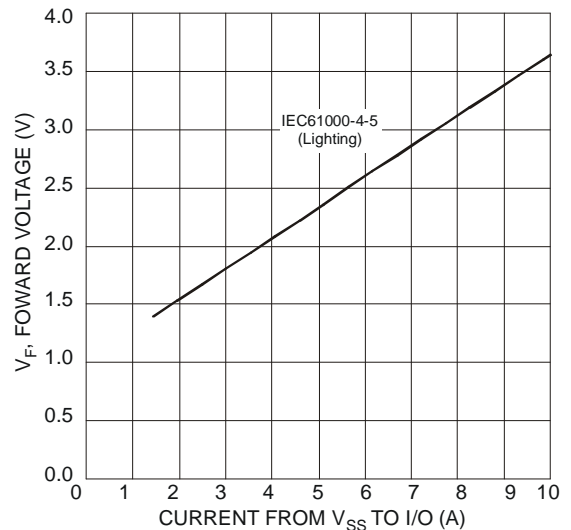
Figure 4 Forward Voltage Characteristic
