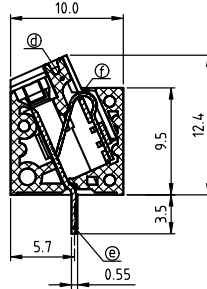
SECTION Q-Q
