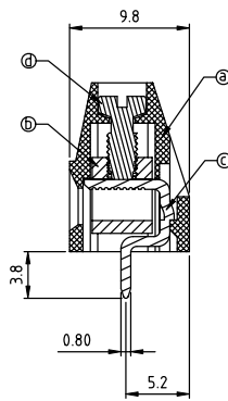
SECTION P-P
