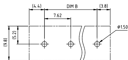
RECOMMENDED P.C.B LAYOUT TOP VIEW
