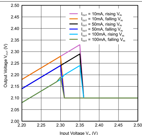
Figure 28. 100% Mode Transition V_{OUT} 2.1V
