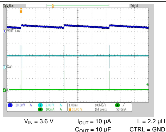
Figure 31. Typical Operation I_{Load} = 10\mu A V_{OUT} = 1.8V
