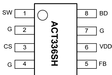
SOP-8 ACT336SH
