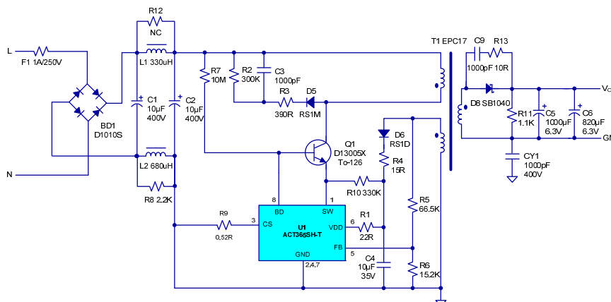
Figure 3: Universal VAC Input, 5V/2.1A Output Adapter
