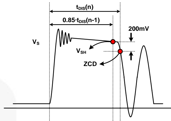
Figure 24. Operation Waveform for ZCD Function
