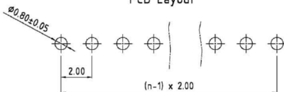
PCB Layout
