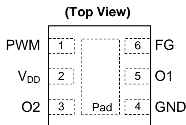
U-DFN2020-6
