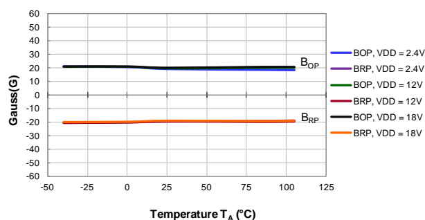
Magnetic Switch Points Bop & Brp vs. Temperature
