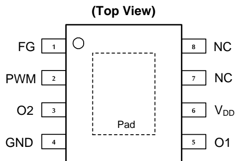
MSOP-8EP
