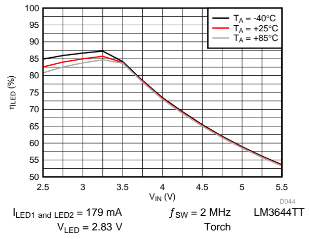
Figure 53. LED Efficiency vs Input Voltage
