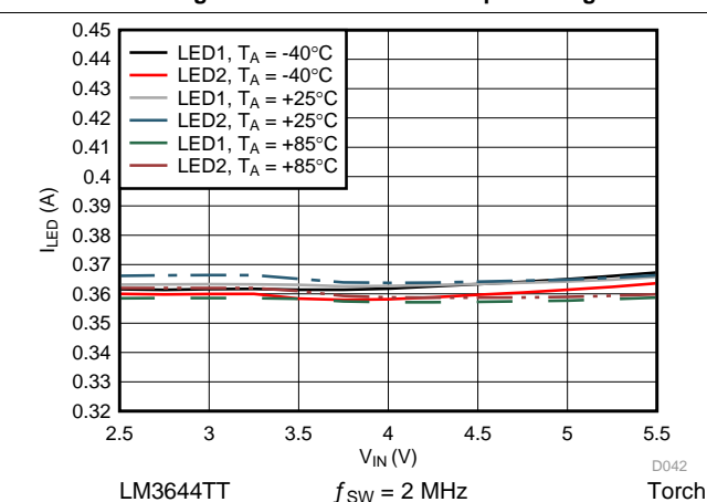
Figure 19. LED Current vs Input Voltage
