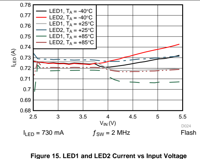
Figure 15. LED1 and LED2 Current vs Input Voltage
