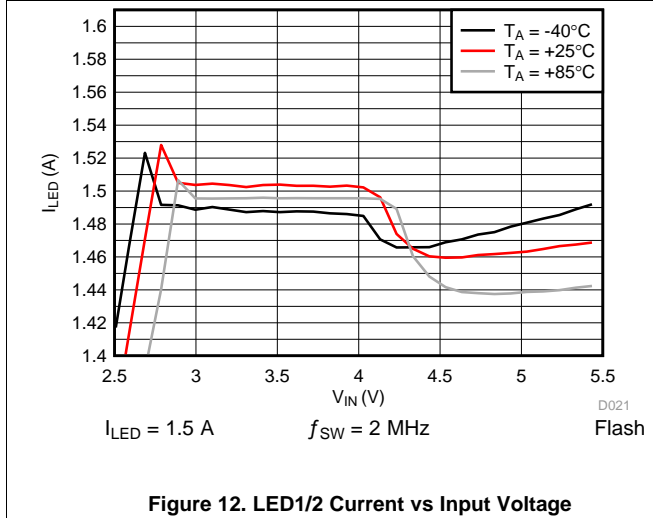
Figure 12. LED1/2 Current vs Input Voltage
