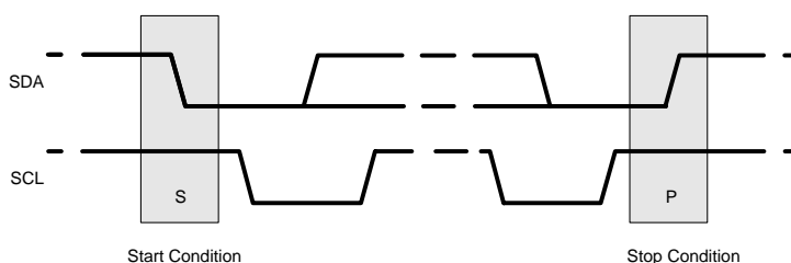
Figure 38. Start and Stop Conditions
