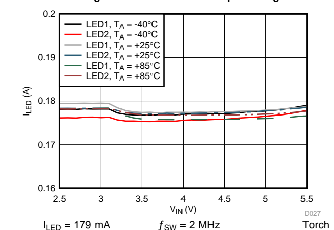
Figure 18. LED Current vs Input Voltage
