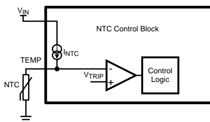
Figure 36. Temp Detection Diagram
