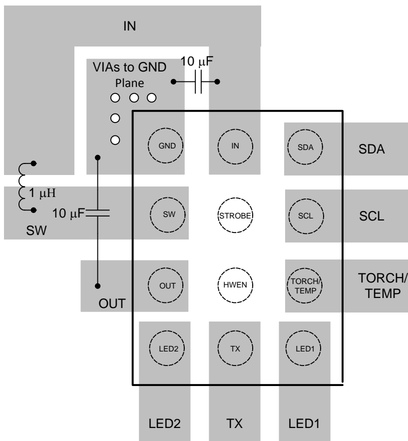
Figure 63. Layout Example
