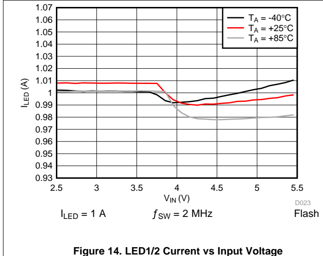
Figure 14. LED1/2 Current vs Input Voltage
