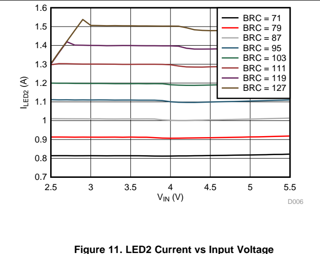
Figure 11. LED2 Current vs Input Voltage
