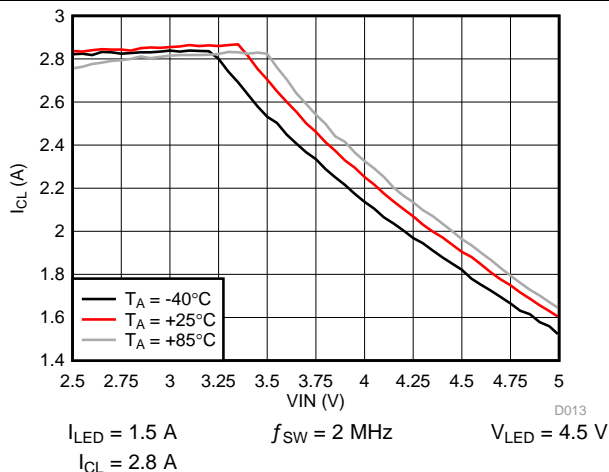
Figure 28. Inductor Current Limit vs Input Voltage
