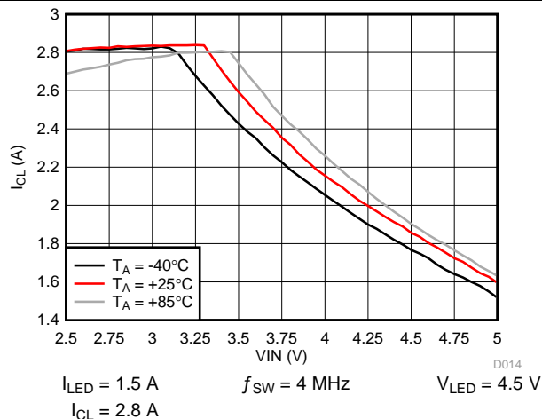
Figure 29. Inductor Current Limit vs Input Voltage
