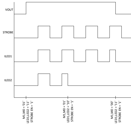
Figure 33. IR Mode Pass Only
