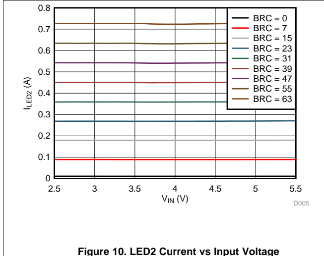
Figure 10. LED2 Current vs Input Voltage
