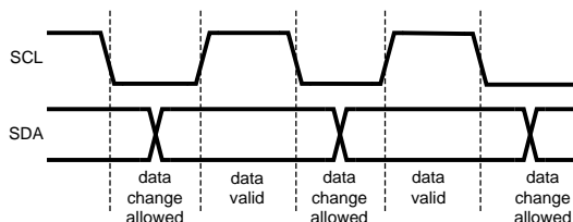
Figure 37. Data Validity Data
