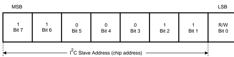
Figure 40. I 2 C-Compatible Chip Address
