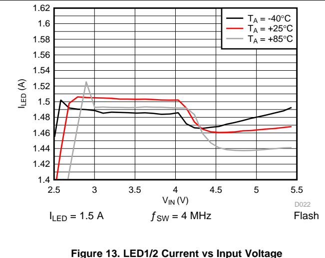
Figure 13. LED1/2 Current vs Input Voltage
