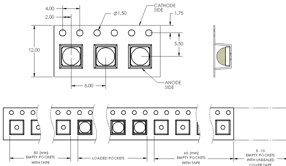
Figure 12: Emitter carrier tape specifications (mm).
