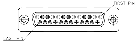
MATING VIEW FOR FEMALE CONNECTOR
