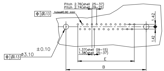
PC card drilling dimensions(after plating) (thickness 1.60±0.20mm)
