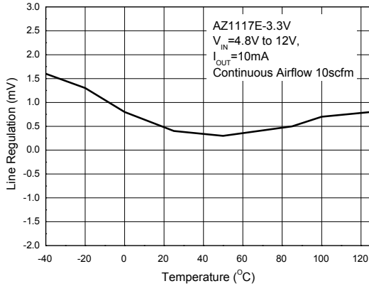
Line Regulation vs. Temperature
