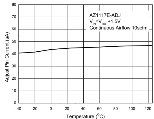
Adjust Pin Current vs. Temperature
