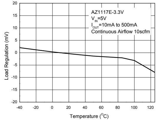
Load Regulation vs. Temperature
