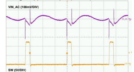
Time-400ns/div
