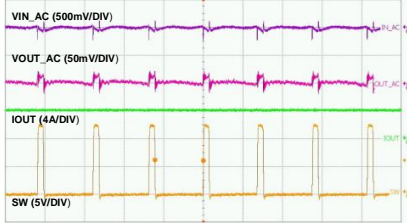
Time-1μs/div
