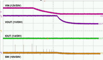
Time-50ms/div
