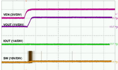
Time-2ms/div
