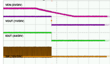
Time-20ms/div
