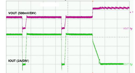
Time-1ms/div
