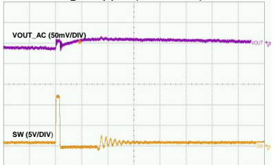
Time-1μs/div
