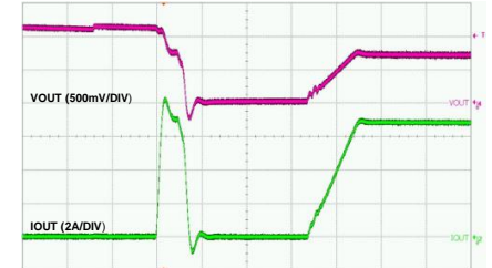
Time-100μs/div
