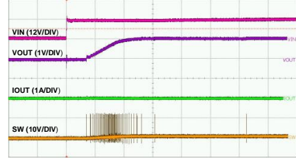
Time-500μs/div
