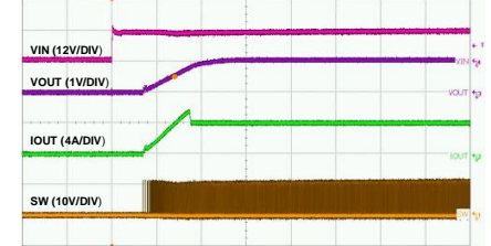
Time-500μs/div
