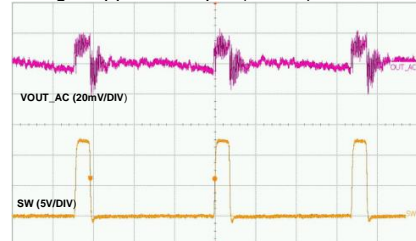
Time-400ns/div
