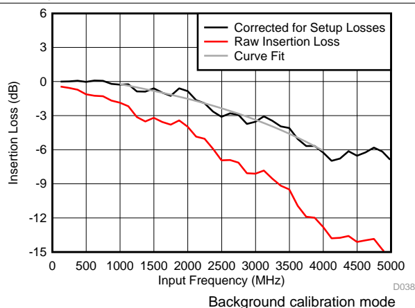
Figure 46. Insertion Loss vs Input Frequency
