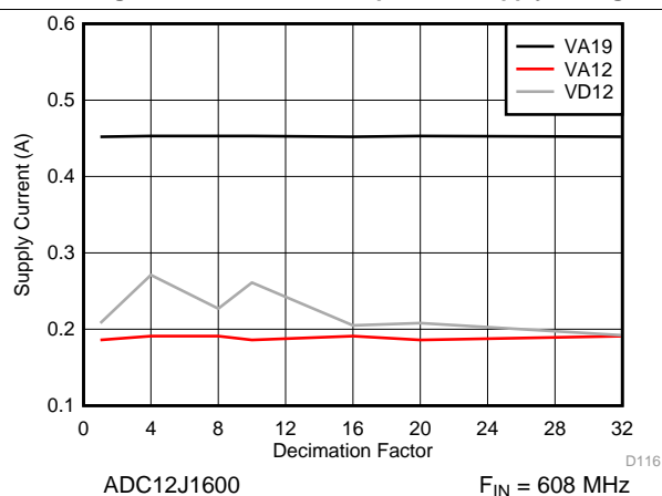
Figure 42. Supply Current vs Decimation Setting
