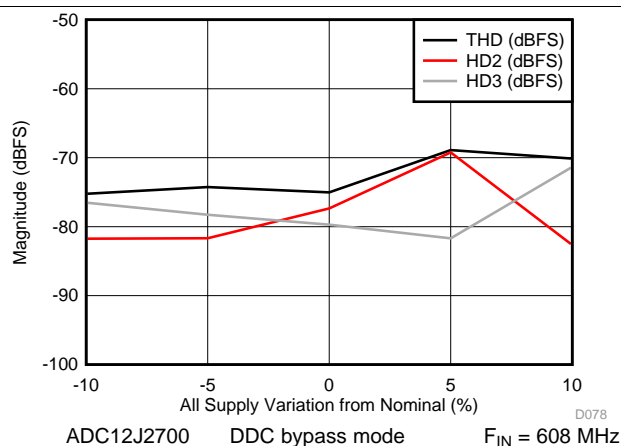
Figure 18. THD, H2, H3 vs Supply Voltage
