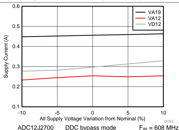
Figure 24. Supply Current vs Supply Voltage
