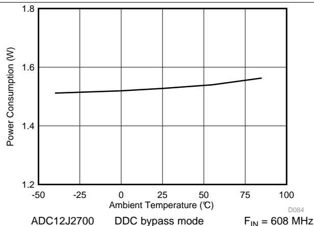
Figure 22. Power Consumption vs Temperature
