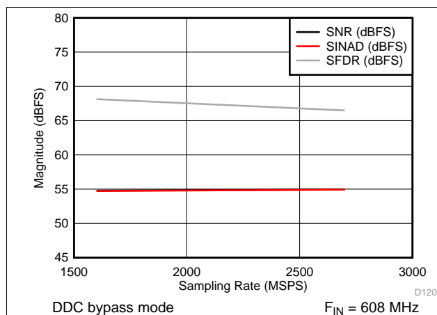
Figure 3. SNR, SINAD, SFDR vs Sampling Rate
