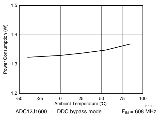
Figure 41. Power Consumption vs Temperature
