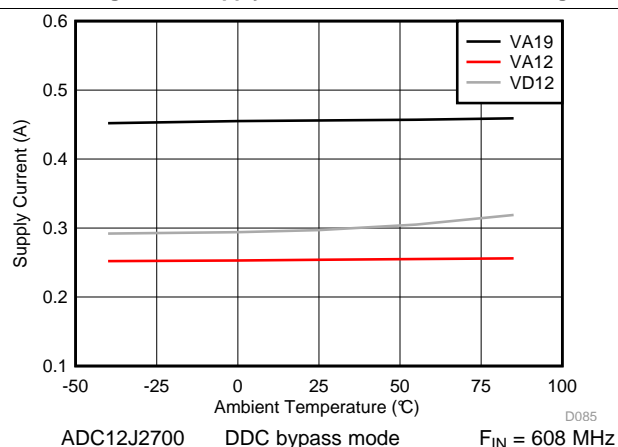
Figure 25. Supply Current vs Temperature
