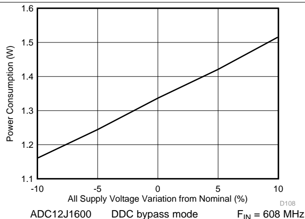
Figure 40. Power Consumption vs Supply Voltage
