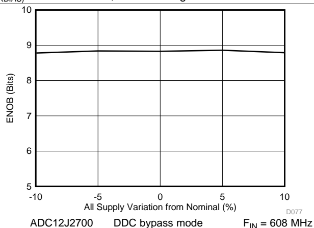
Figure 15. ENOB vs Supply Voltage
