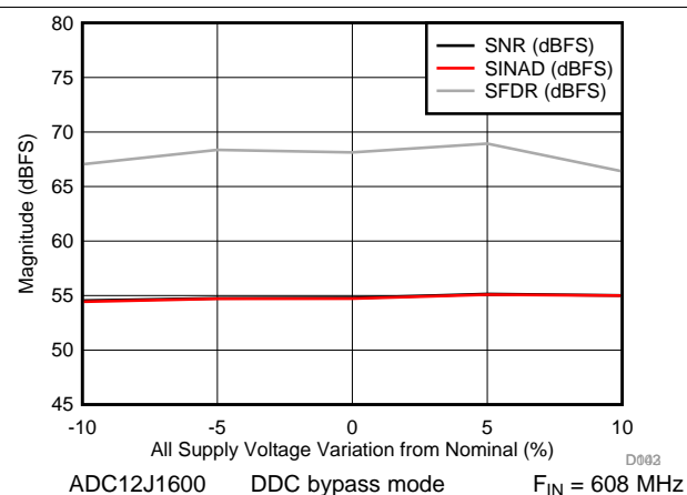
Figure 29. SNR, SINAD, SFDR vs Supply Voltage
