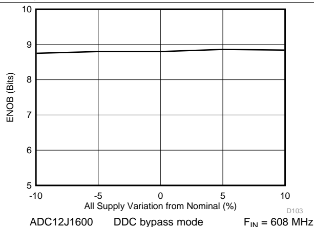
Figure 34. ENOB vs Supply Voltage
