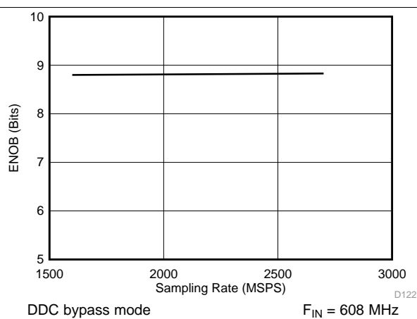
Figure 4. ENOB vs Sampling Rate
