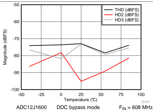
Figure 38. THD, H2, H3 vs Temperature
