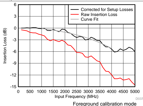
Figure 45. Insertion Loss vs Input Frequency
