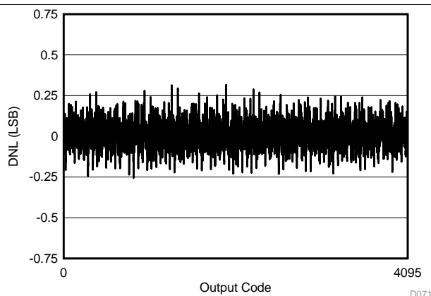
Figure 47. DNL versus Code - ADC12J2700
