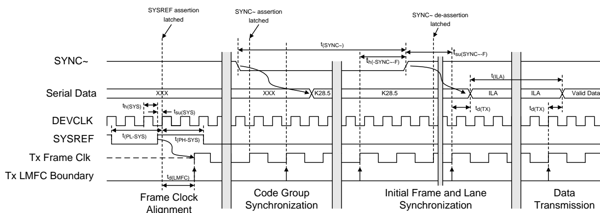
Figure 1. JESD204 Synchronization
