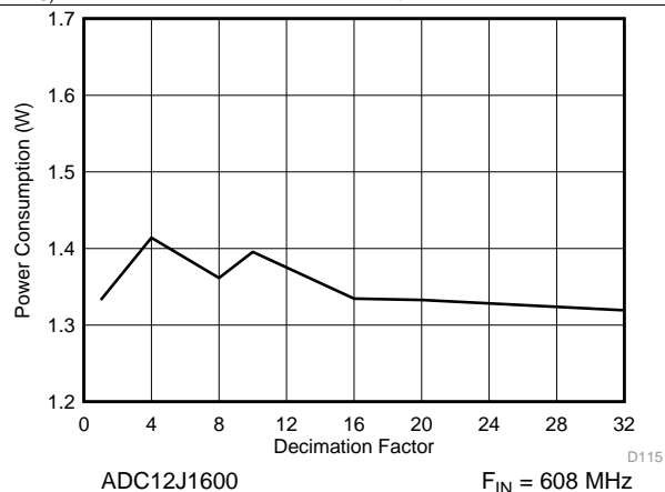
Figure 39. Power Consumption vs Decimation Setting
