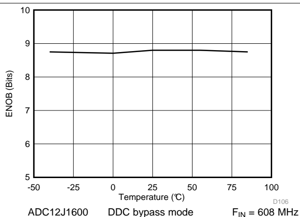
Figure 35. ENOB vs Temperature
