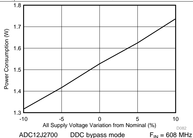
Figure 21. Power Consumption vs Supply Voltage
