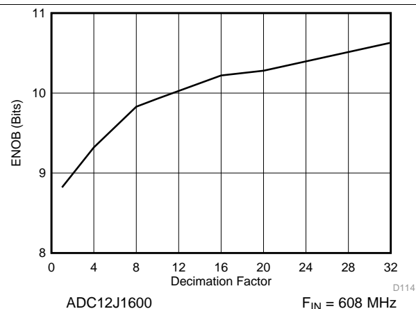
Figure 32. ENOB vs Decimation Setting
