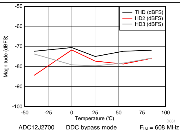
Figure 19. THD, H2, H3 vs Temperature
