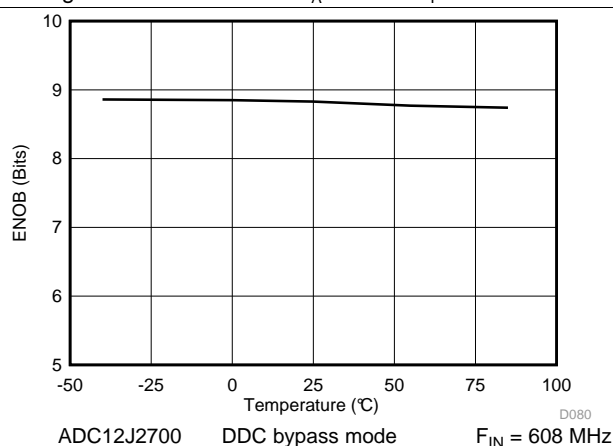
Figure 16. ENOB vs Temperature ADC12J2700
