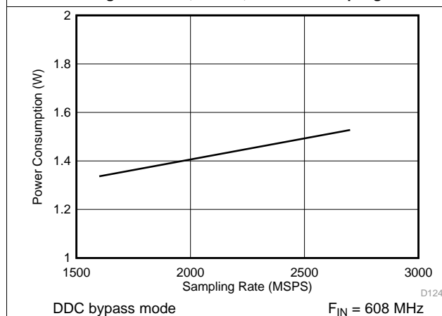
Figure 5. Power Consumption vs Sampling Rate
