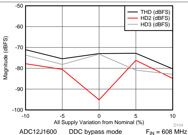
Figure 37. THD, H2, H3 vs Supply Voltage
