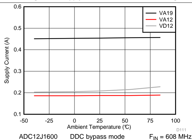
Figure 44. Supply Current vs Temperature
