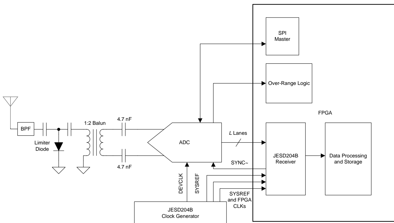
Figure 109. Simplified Schematic
