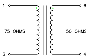
SCHEMATIC
