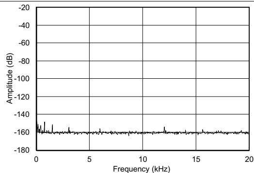
Figure 15. 2 FFT Plot at BPZ With Amute
