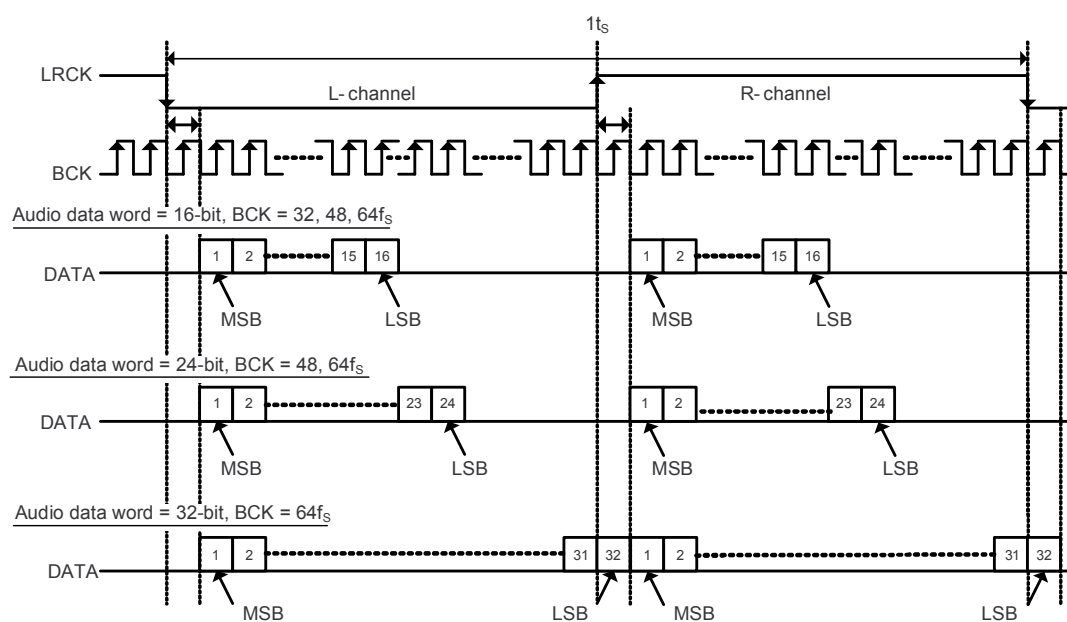
Figure 19. I 2 S Audio Data Format
