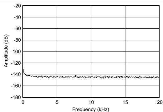
Figure 11. 2 FFT Plot At -60db Input
