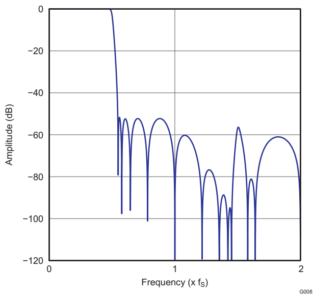
Figure 36. Low latency x4 Interpolation Filter Frequency Response
