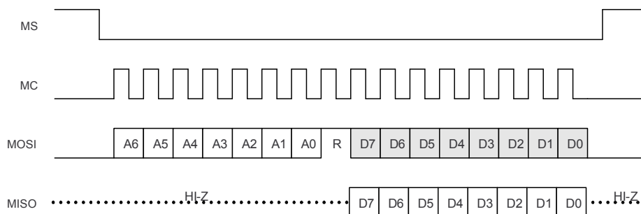
Figure 74. Serial Control Format; Read
