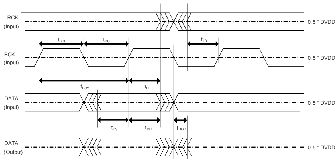
Figure 5. PCM5242 Serial Audio Timing - Slave
