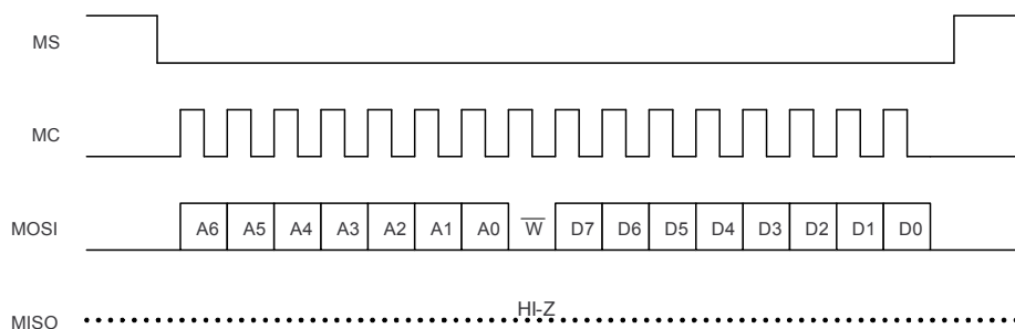
Figure 72. Serial Control Format; Write, Single Byte
