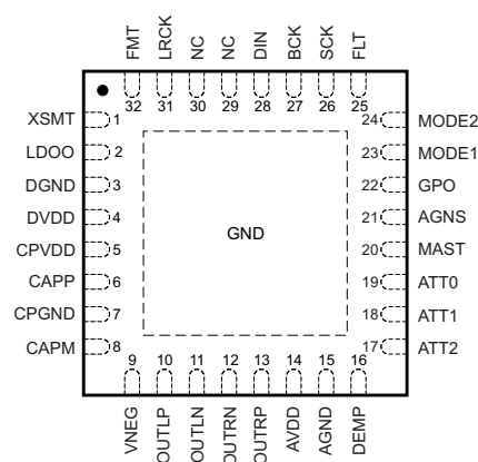
Figure 3. Hardware Control
