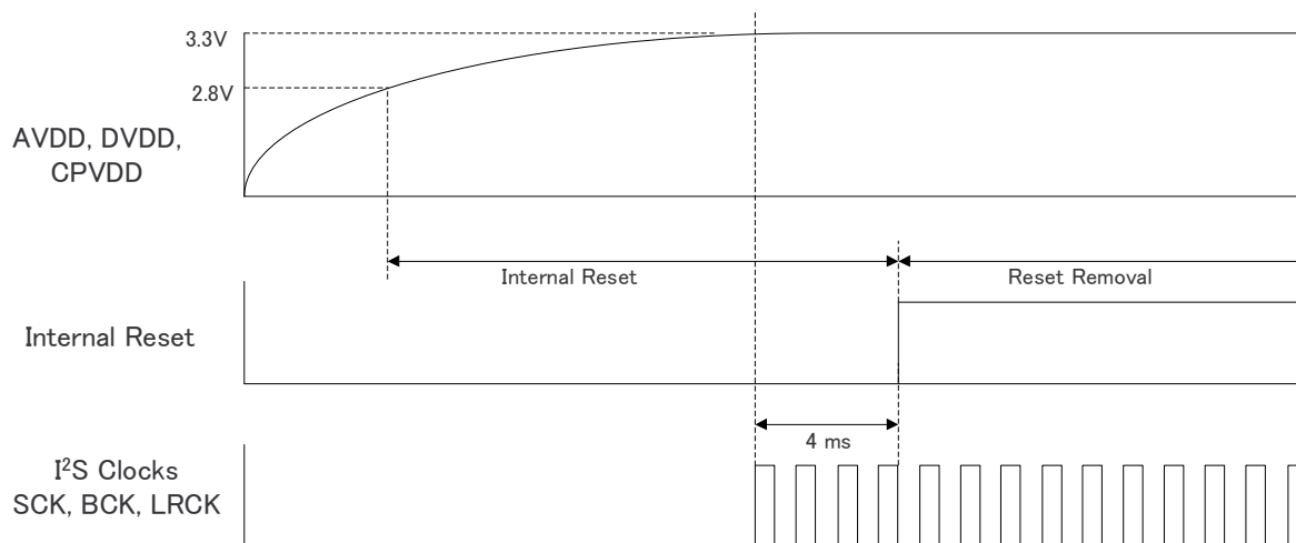
Figure 86. Power-On Reset Timing, DVDD = 3.3V
