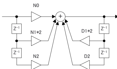
Figure 62. Biquad Block
