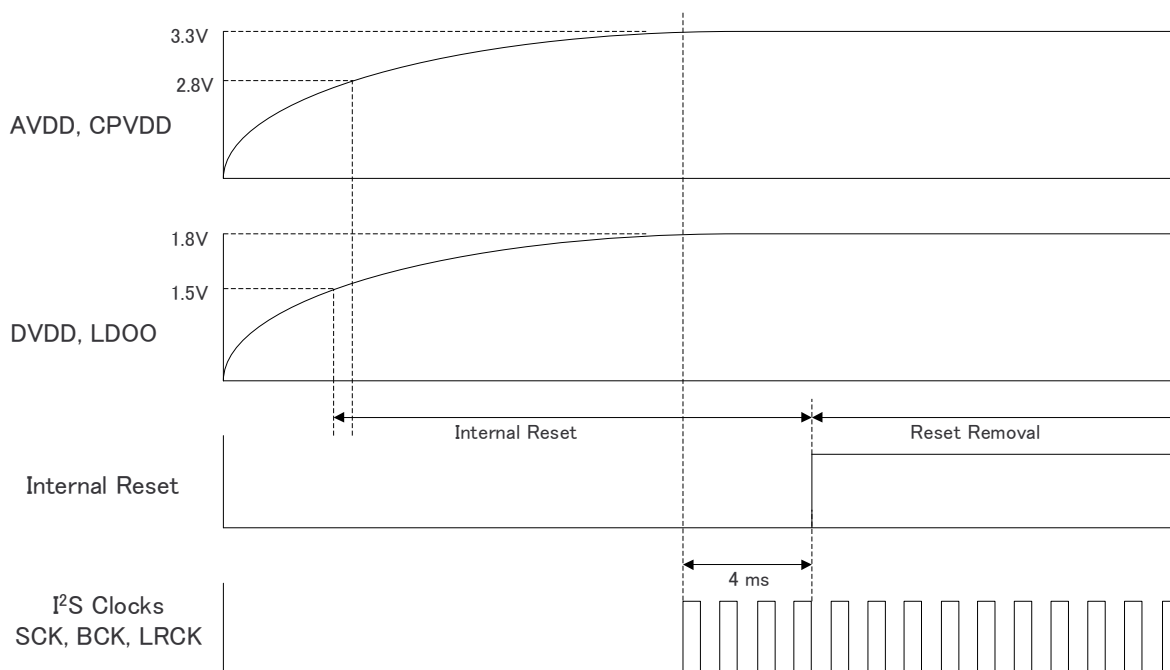
Figure 87. Power-On Reset Timing, DVDD = 1.8V
