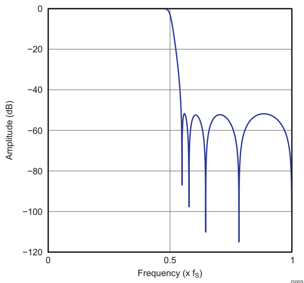
Figure 39. Low latency x2 Interpolation Filter Frequency Response
