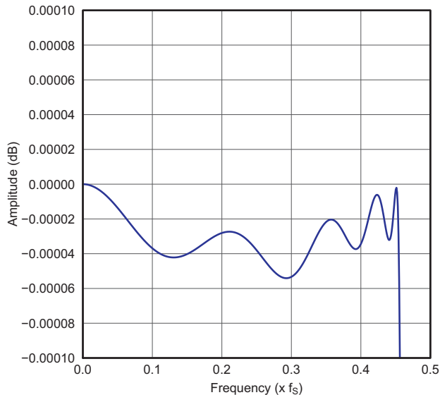
Figure 35. Low latency x8 Interpolation Filter Passband Ripple
