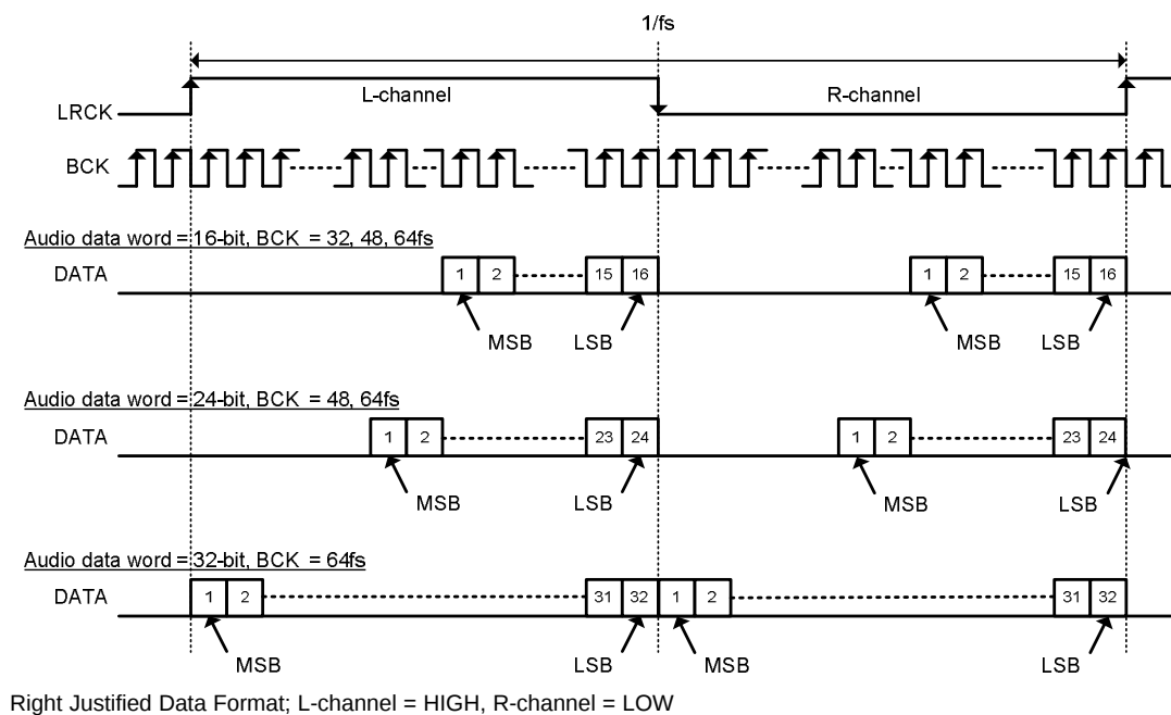
Figure 20. Right Justified Audio Data Format
