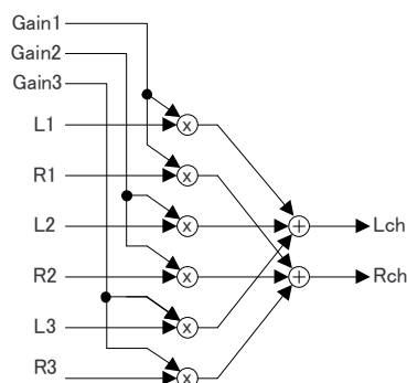
Figure 63. Stereo Mixer Block
