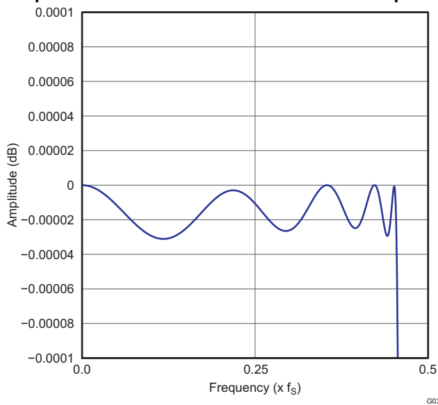
Figure 38. Low latency x4 Interpolation Filter Passband Ripple
