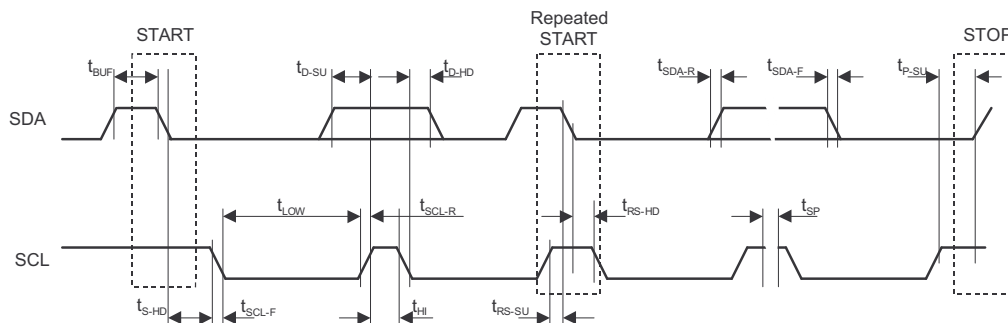
Figure 79. Register Access Timing
