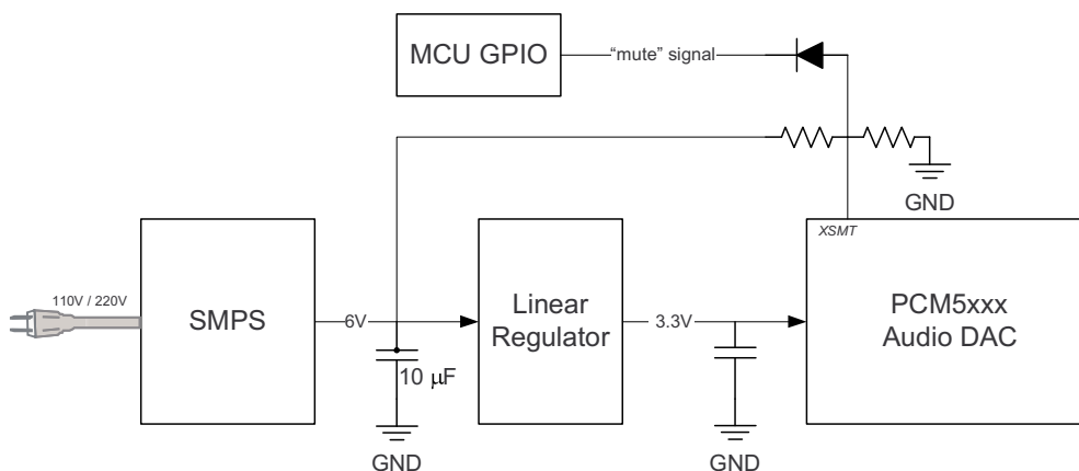
Figure 83. Using the XSMT Pin
