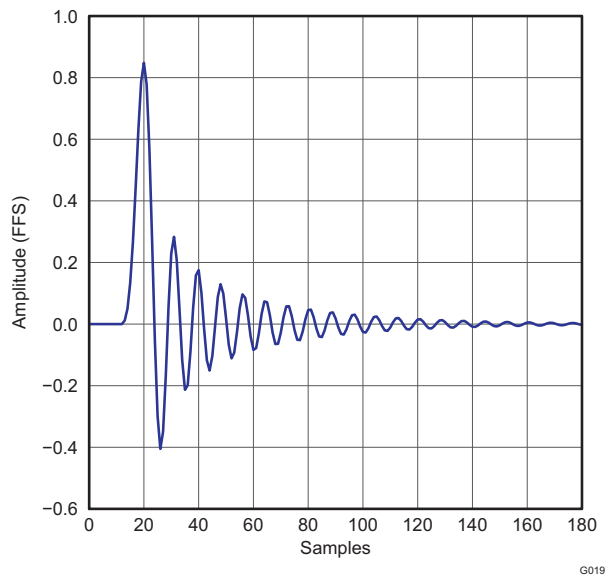
Figure 37. Low latency x4 Interpolation Filter Impulse Response
