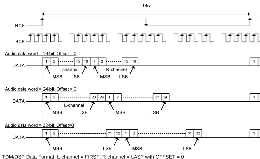
Figure 21. TDM/DSP 1 Audio Data Format
