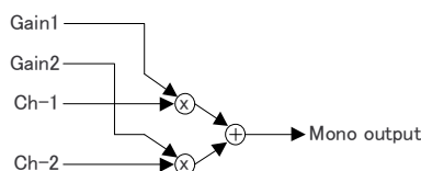
Figure 65. Mono Mixer Block
