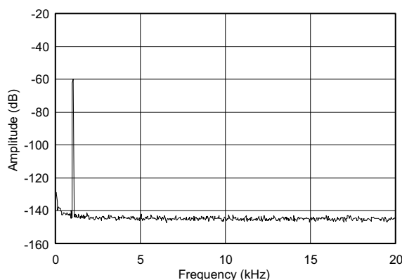
Figure 81. 2 FFT Plot At -60db Input
