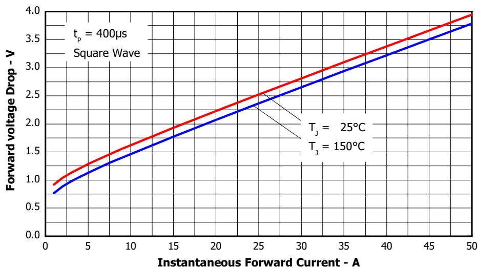
Figure 11. Maximum Forward voltage Drop (Input Bridge Rectifier)
