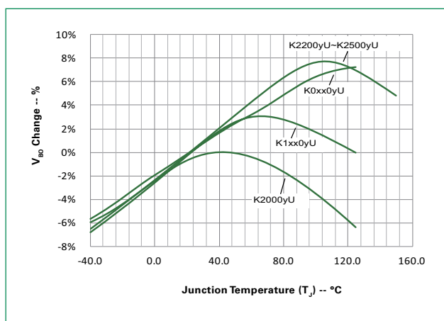
Figure 7: Normalized V_{BO} Change vs. Junction Temperature
