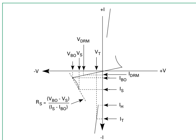
Figure 1: V-I Characteristics
