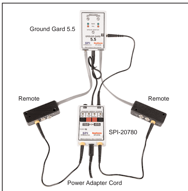
Figure 5. Connecting the Ground Gard Verifier to the Ground Gard 5.5
