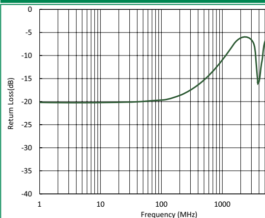
Differential Return Loss SDD22 vs. Frequency ( Z_{diff} = 100\Omega )
