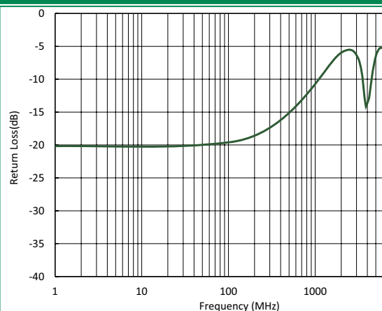
Differential Return Loss SDD11 vs. Frequency ( Z_{diff} = 100\Omega )
