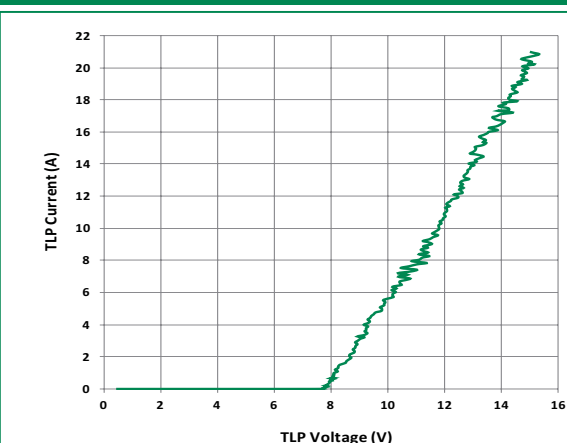
Transmission Line Pulsing (TLP) Plot
