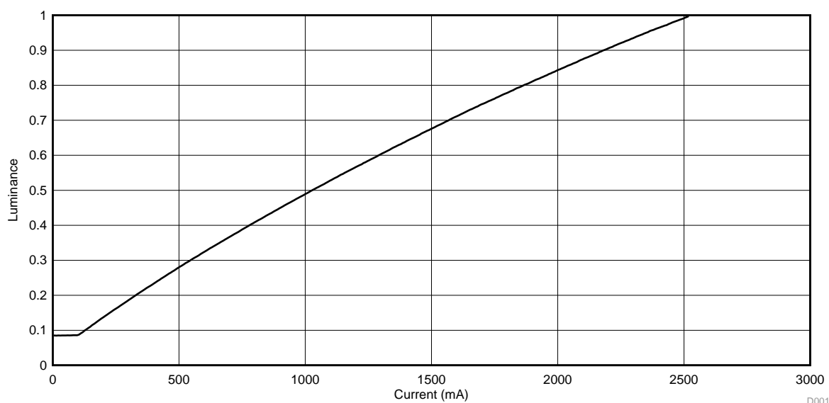
Figure 16. Luminance vs Current
