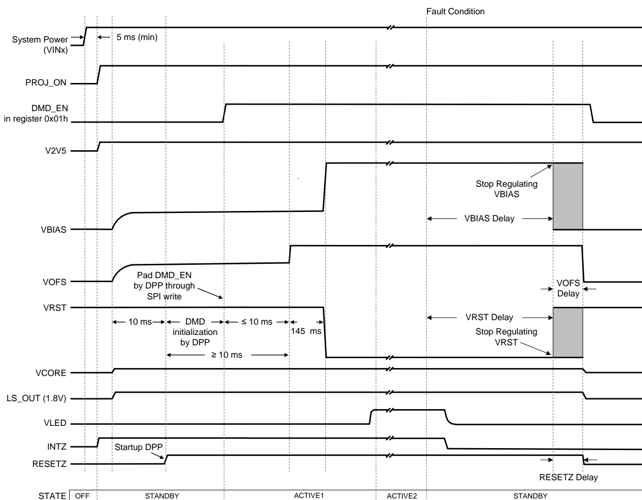
Figure 4. Power Sequence Fault Shutdown Mode
