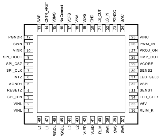
DLPA2005 VQFN Package (BOTTOM VIEW)
