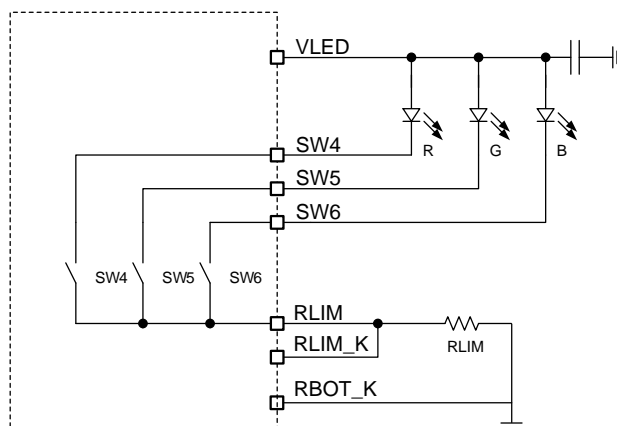
Figure 5. Switch Connection for a Common-Anode LED Assembly
