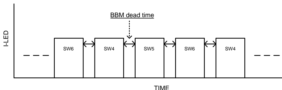
Figure 6. BBM Timing (See Register 0Bh in Table 20)
