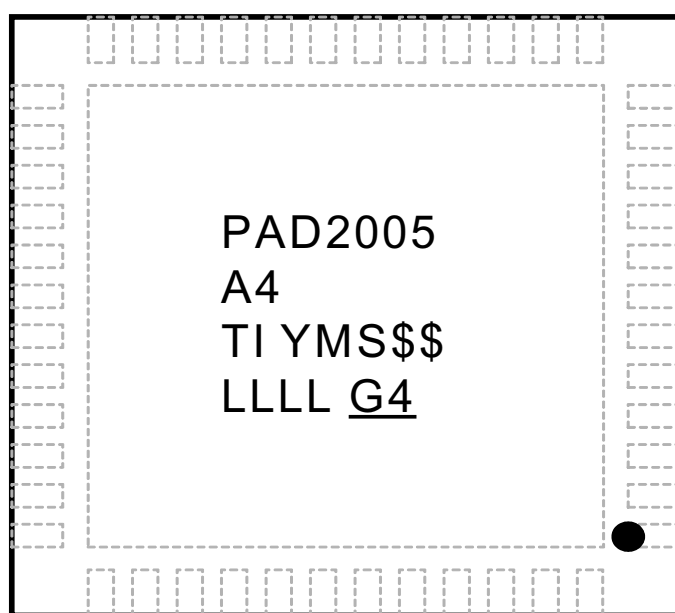
Figure 20. Package Marking DLPA2005 (Top View)
