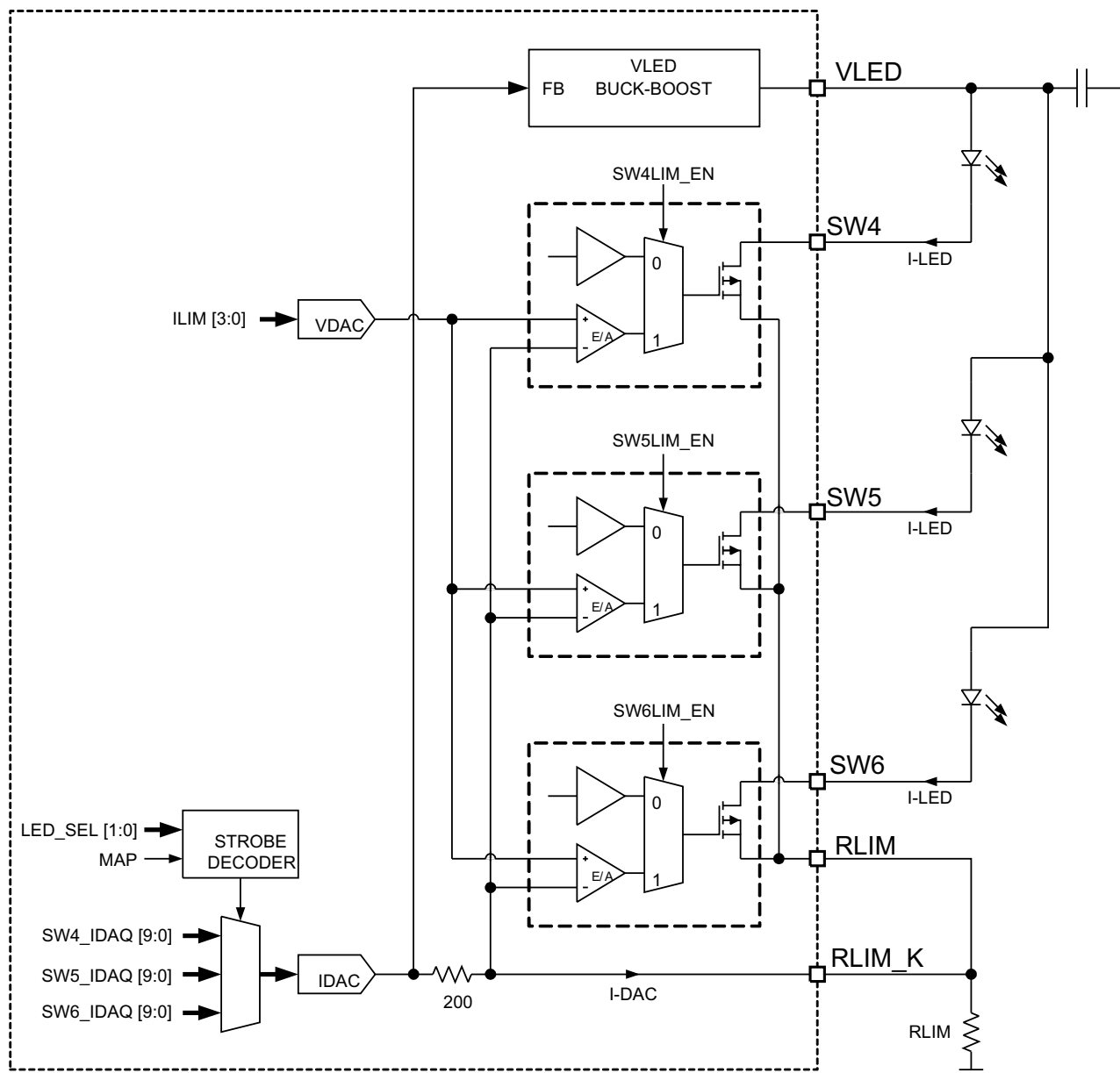
Figure 9. LED Driver Block Diagram
