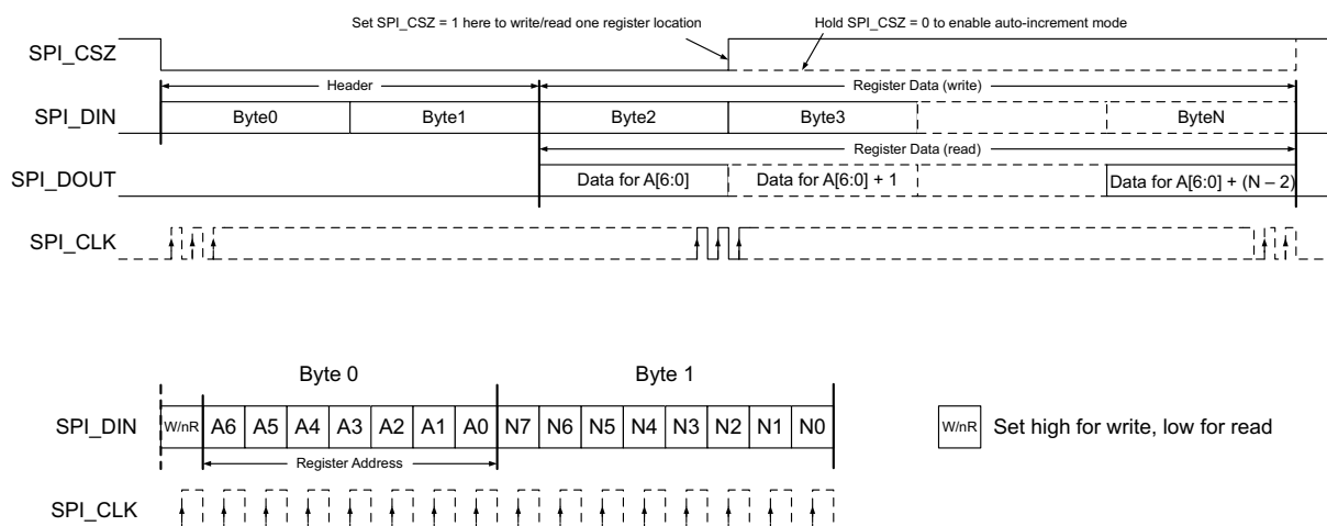
Figure 13. SPI Protocol
