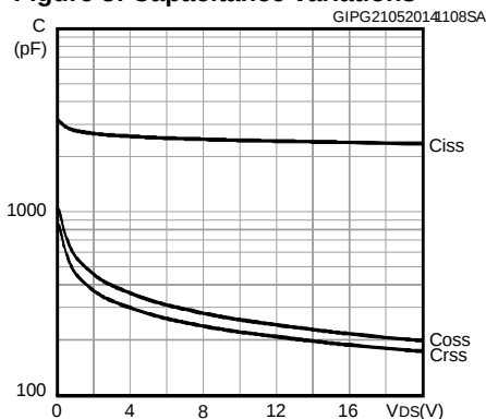
Figure 8: Capacitance variations
