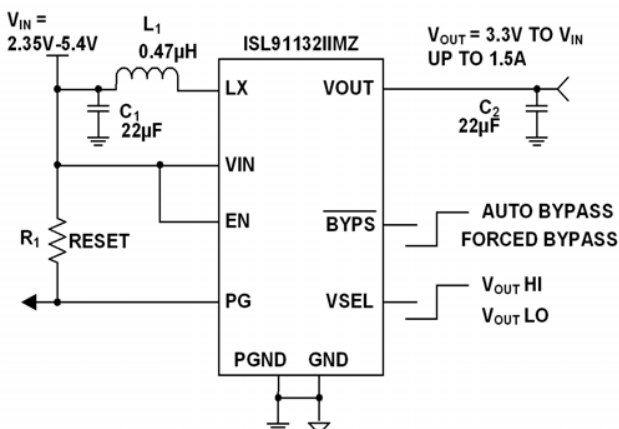
FIGURE 1. TYPICAL APPLICATION
