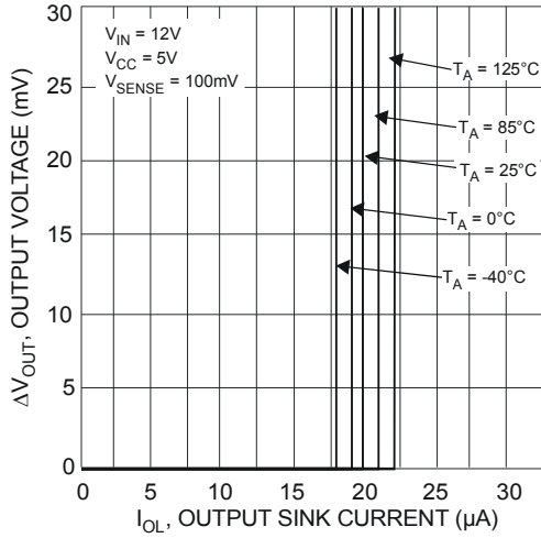
Fig. 7 Output Current Sink
