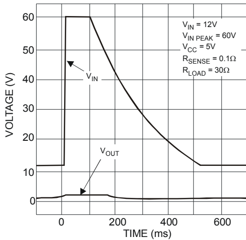
Fig. 16 Load Dump Waveform
