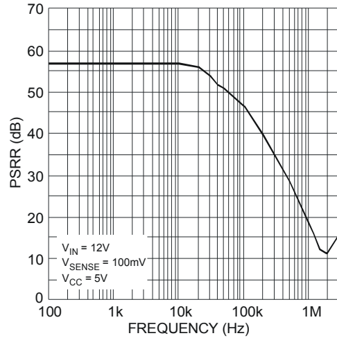
Fig. 19 Supply Rejection
