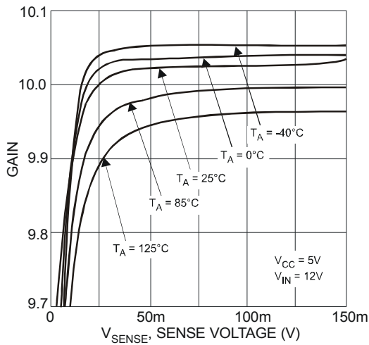
Fig. 9 Differential gain
