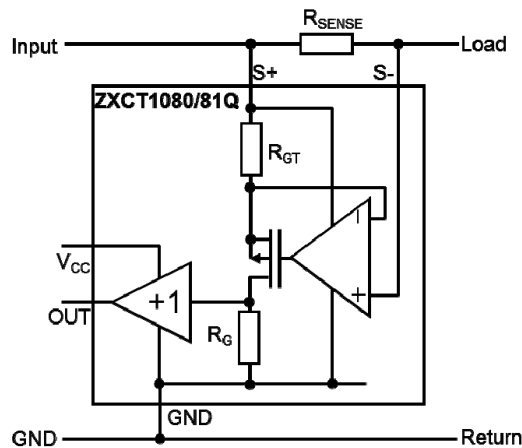
Fig. 20 Typical Configuration of ZXCT1080Q/81Q
