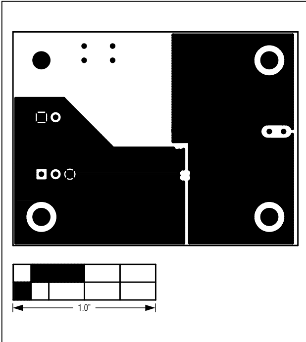
Figure 5. MAX8989 EV Kit PCB Layout—Inner Layer 3
