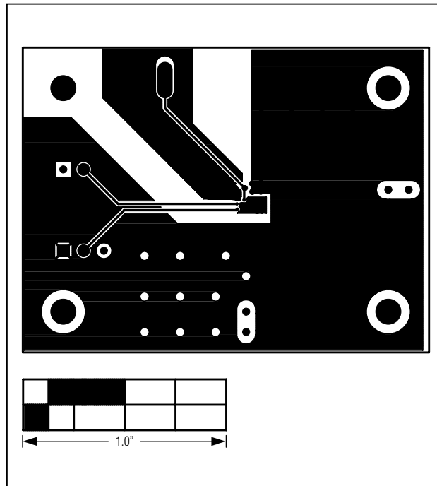
Figure 4. MAX8989 EV Kit PCB Layout—Inner Layer 2
