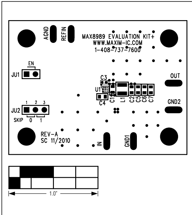
Figure 2. MAX8989 EV Kit Component Placement Guide—Component Side
