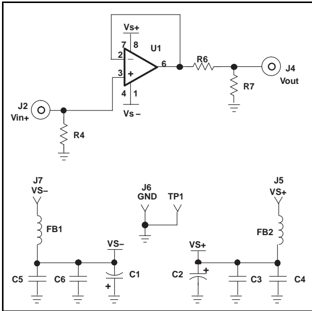
Figure 100. THS4271 Unity Gain EVM Circuit Configuration
