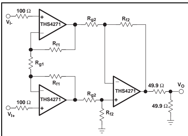
Figure 84. A High-Speed Instrumentation Amplifier
