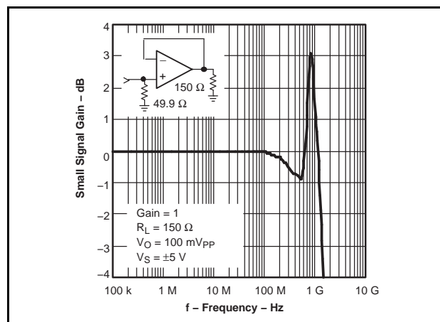
Figure 94. Frequency Response Using the EDGE #6443547 EVM
