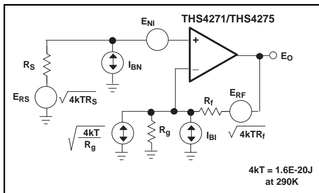
Figure 87. Noise Analysis Model
