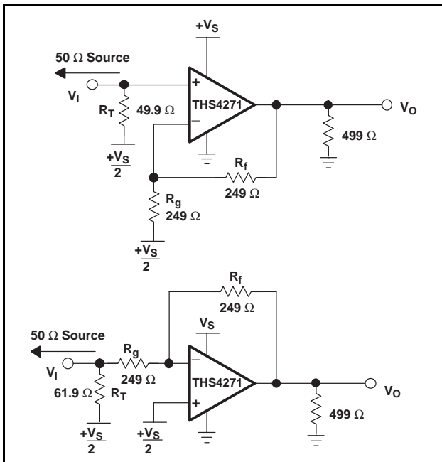
Figure 77. DC-Coupled Single-Supply Operation
