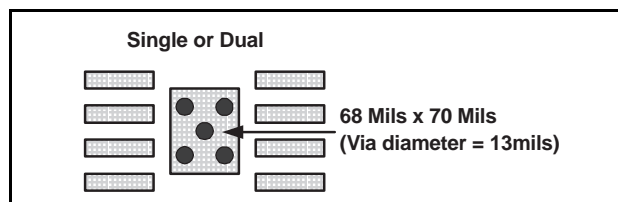
Figure 90. PowerPAD PCB Etch and Via Pattern
