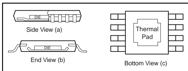
Figure 89. Views of Thermally Enhanced Package
