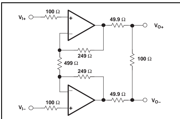
Figure 83. A High Input Impedance, Low-Noise, Differential Receiver
