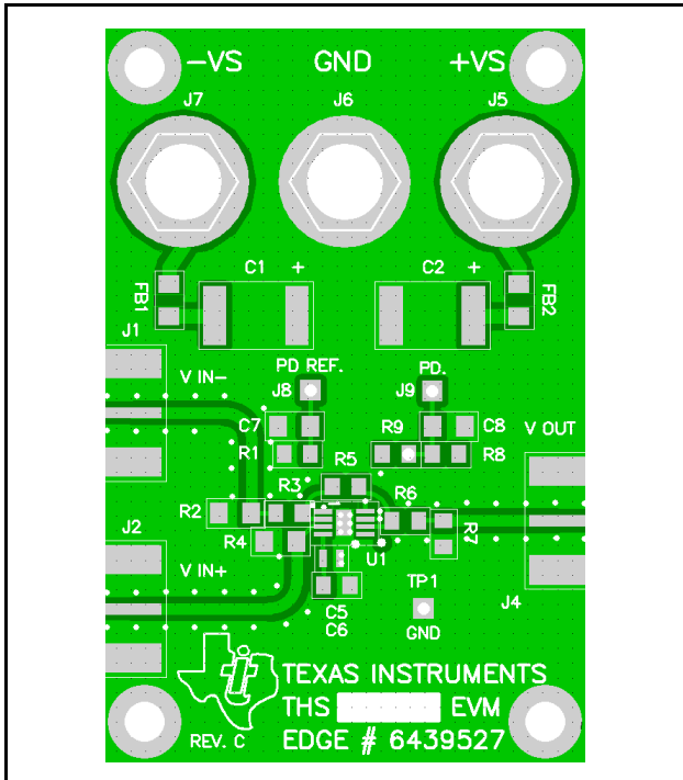
Figure 96. THS4271/THS4275 EVM Board Layout (Top Layer)
