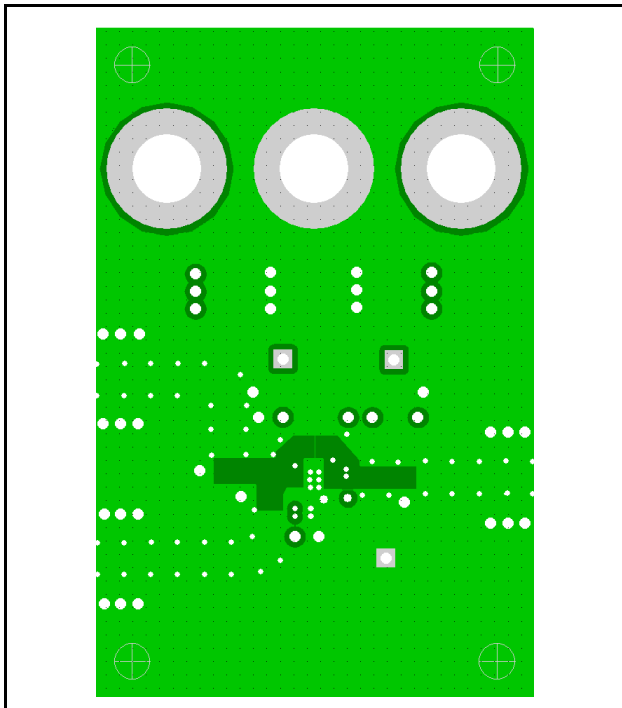
Figure 97. THS4271/THS4275 EVM Board Layout (Second Layer, Ground)
