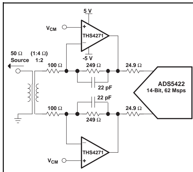
Figure 78. A Linear, Low-Noise, High-Gain ADC Preamplifier
