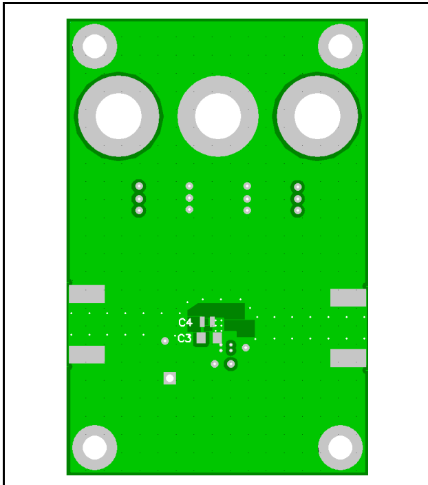
Figure 104. THS4271 Unity Gain EVM Board Layout
