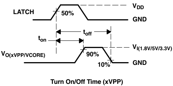
Figure 1. Test Circuits and Voltage Waveforms
