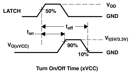
Figure 1. Test Circuits and Voltage Waveforms
