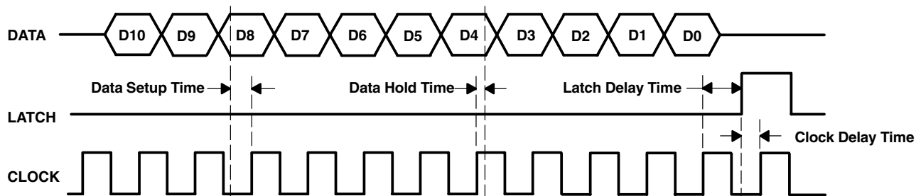
Figure 2. Serial-Interface Timing for TPS2228/TPS2221 Power Interface Switch
