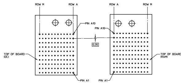
COPLANAR MATED SIGNAL PATHS
