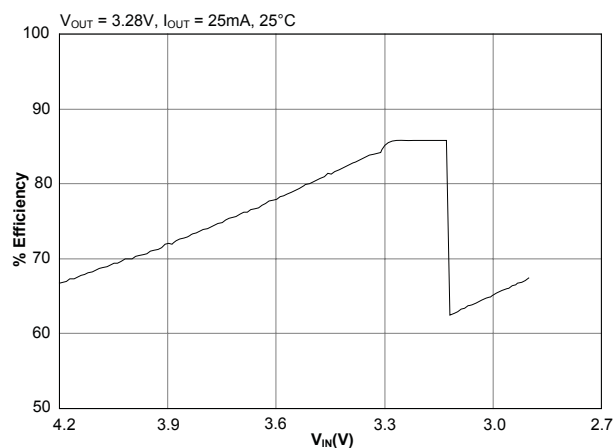
Backlight Efficiency (5 LEDs) — 5.0mA Each
