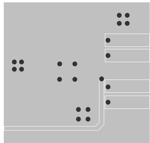
Figure 4 — Layer 2
