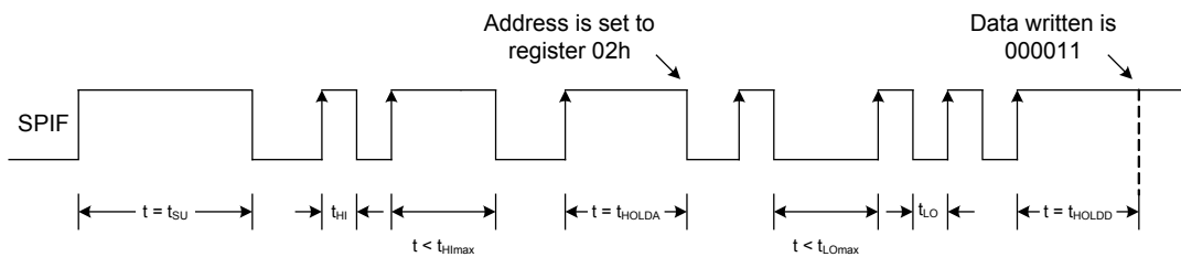
Figure 6 — SemPulse Data Write with Non-Uniform Pulse Widths
