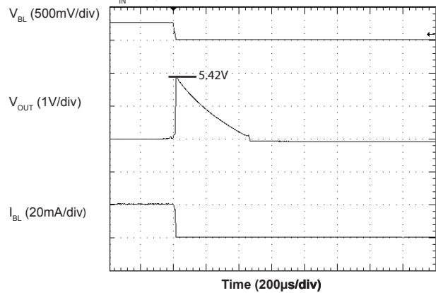
Output Open Circuit Protection
