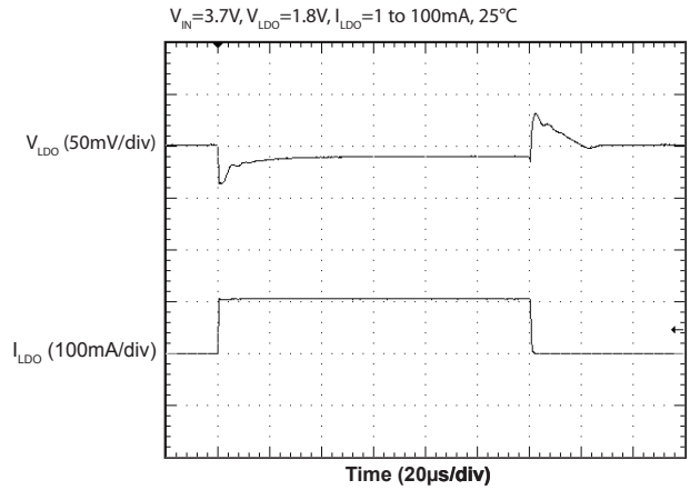
LDO Load Transient Response (1.8V)
