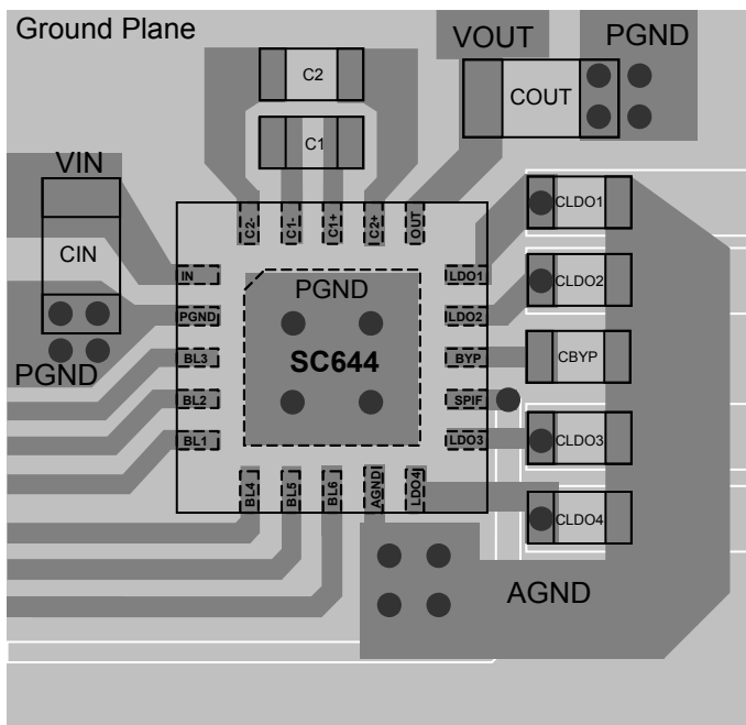
Figure 2 — Recommended PCB Layout
