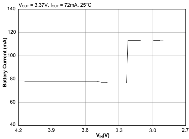
Battery Current (6 LEDs) — 12mA Each
