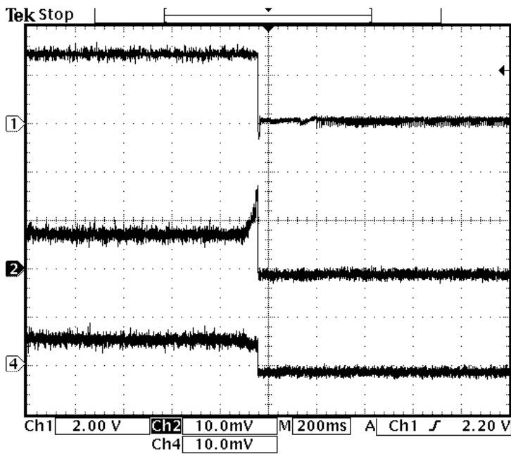
Figure 2: V_{OUT} vs I_{IN(5V)} and I_{IN(12V)} with V_{CC} removed and 4A load. Soft start capacitor = 10nF.
