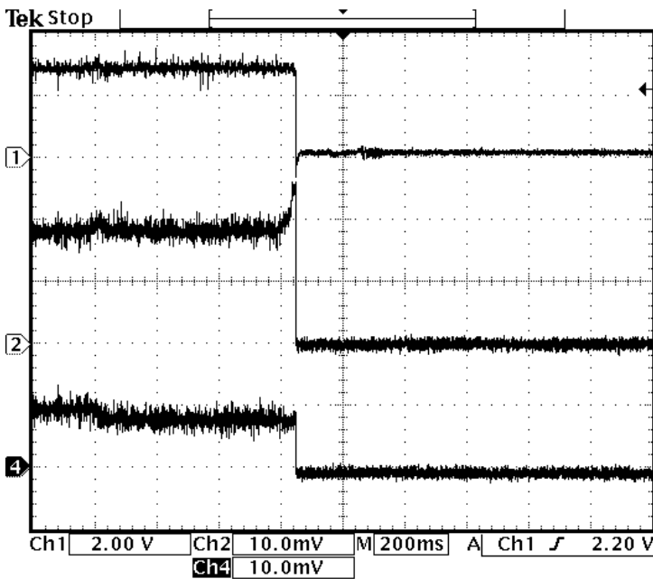
Figure 4: V_{OUT} vs I_{IN(5V)} and I_{IN(12V)} with V_{CC} removed and 12A load. Soft start capacitor = 10nF.
