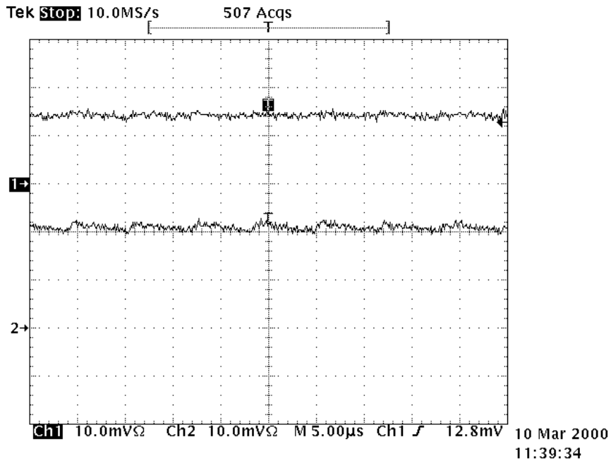
Figure 7: Output Current
