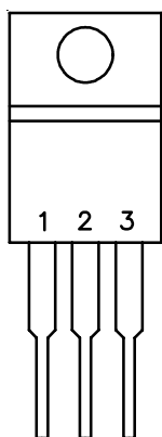
TO-220-3
