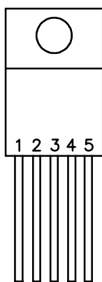
TO-220-5
