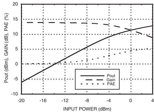
Power Compression @ 4 GHz
