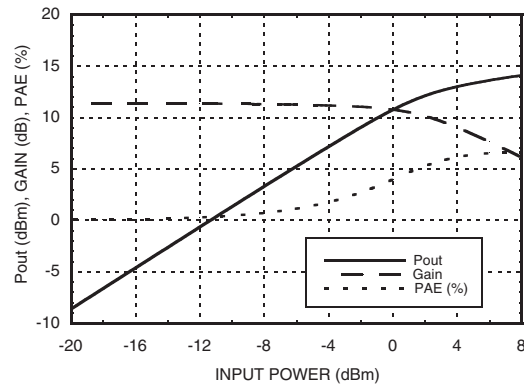
Power Compression @ 8 GHz
