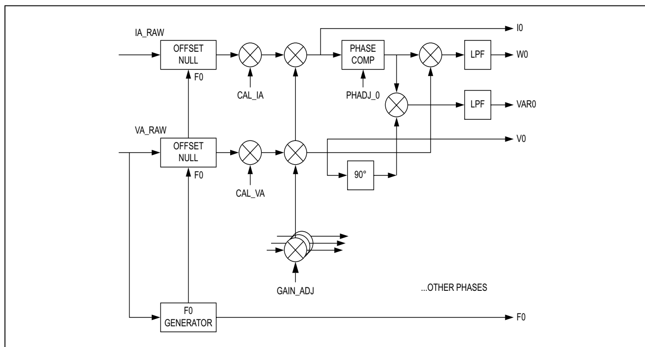
Figure 21. CE Data Flow—Offset, Gain, and Phase Compensation
