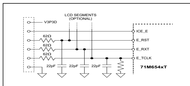
Figure 19. Typical Emulator Connections
