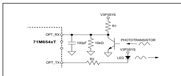
Figure 18. Optical Interface Typical Operating Circuit
