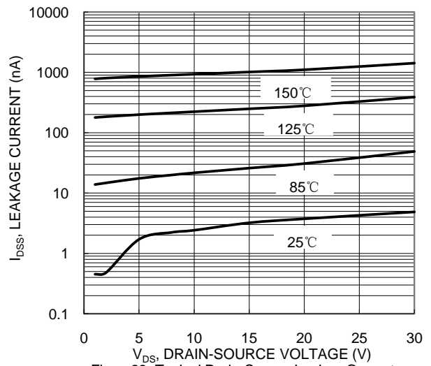
Figure 23. Typical Drain-Source Leakage Current vs Voltage
