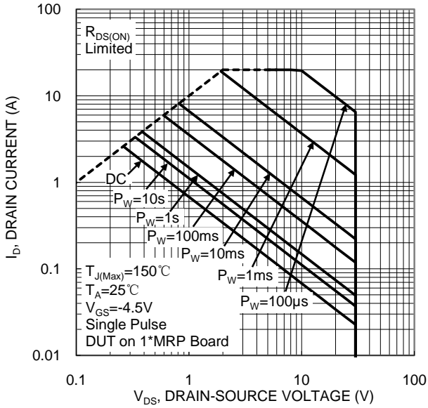
Figure 26. SOA, Safe Operation Area
