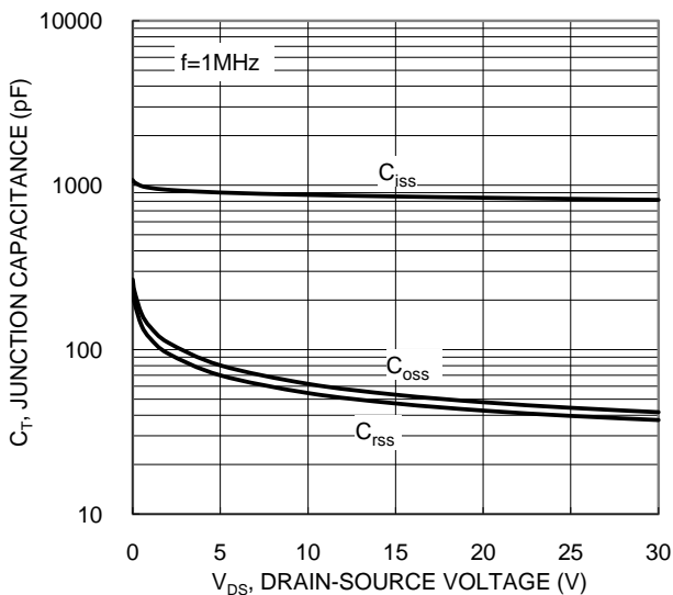
Figure 24. Typical Junction Capacitance
