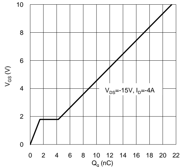
Figure 25. Gate Charge
