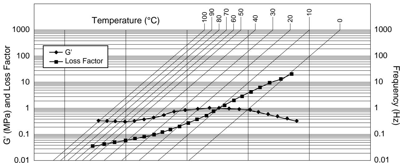
242 Viscoelastic Damping Polymer Nomograph
