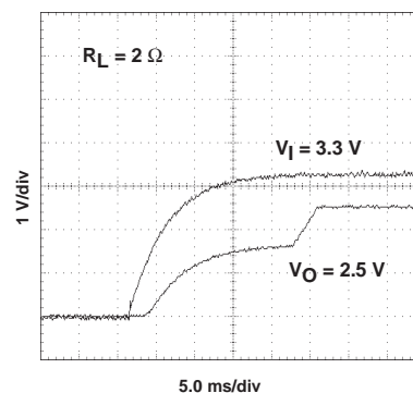
START UP WAVEFORM
