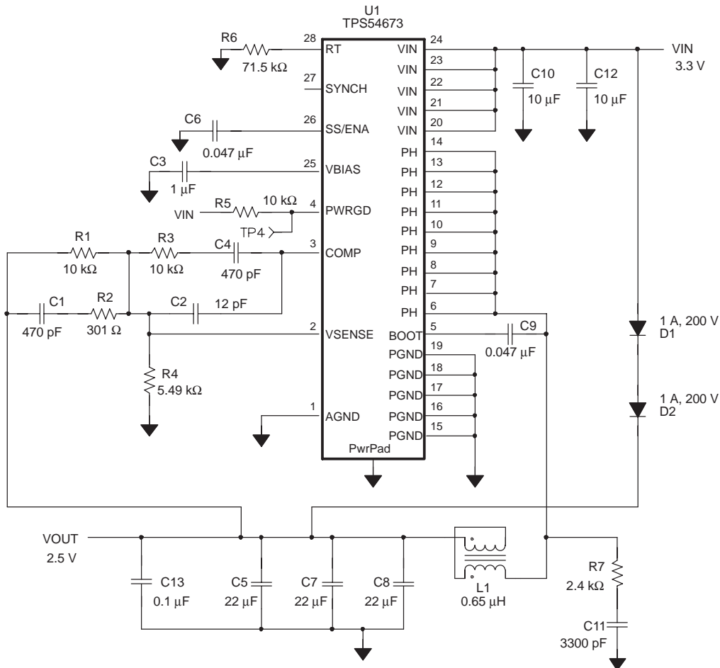
Figure 10. Application Circuit
