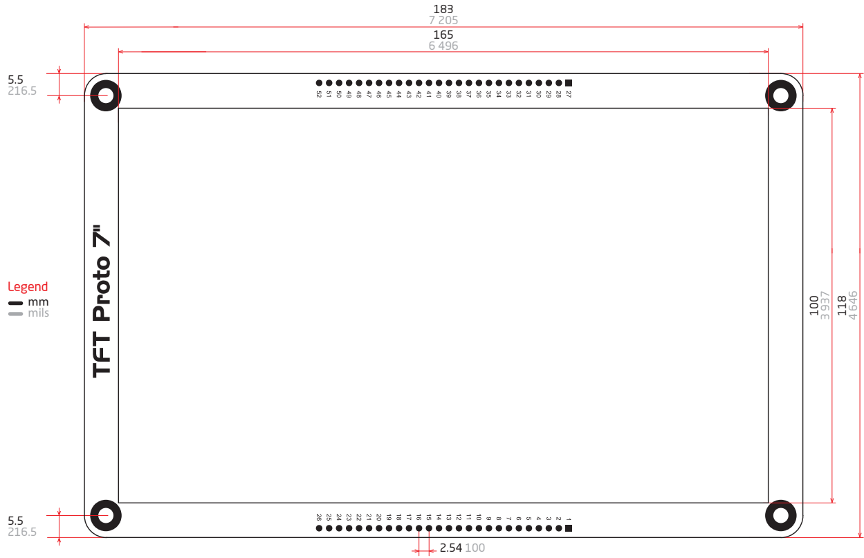
Figure 4: Board dimensions
