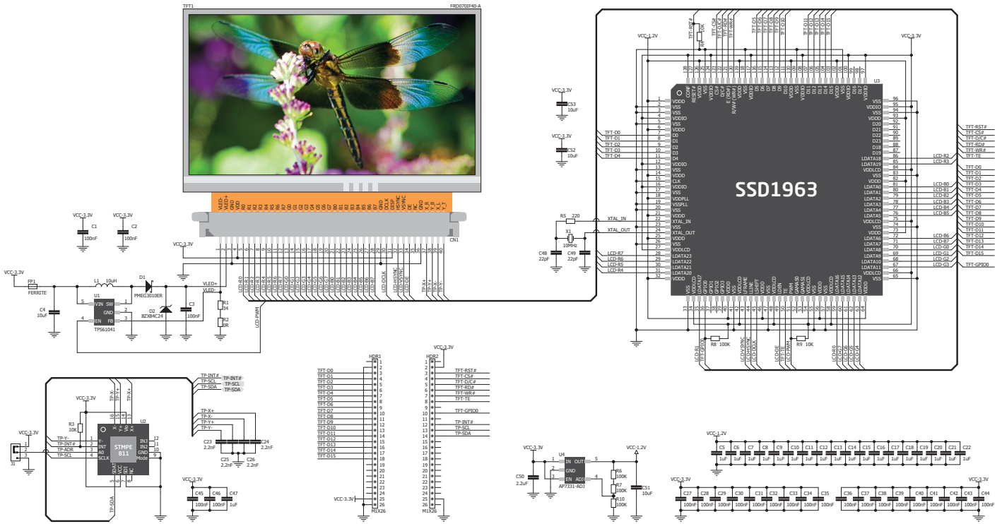
Figure 2: TFT Proto 7" schematic
