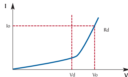
LED I-V Curve
