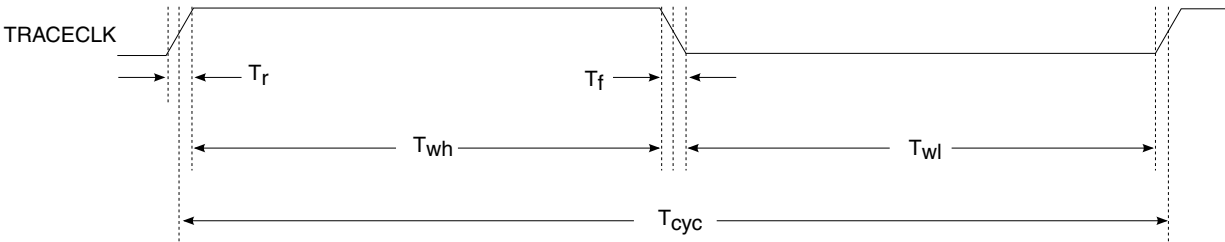
Figure 5. TRACE_CLKOUT specifications
