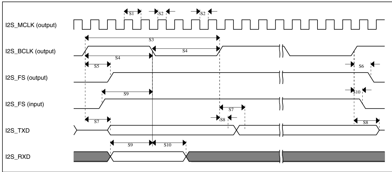
Figure 26. I 2 S timing — master mode
