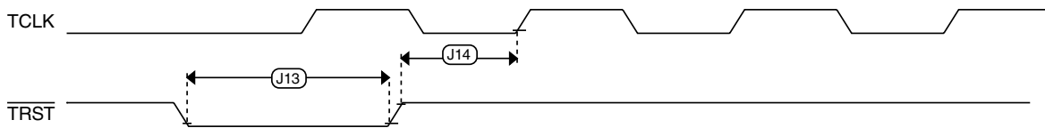
Figure 10. TRST timing
