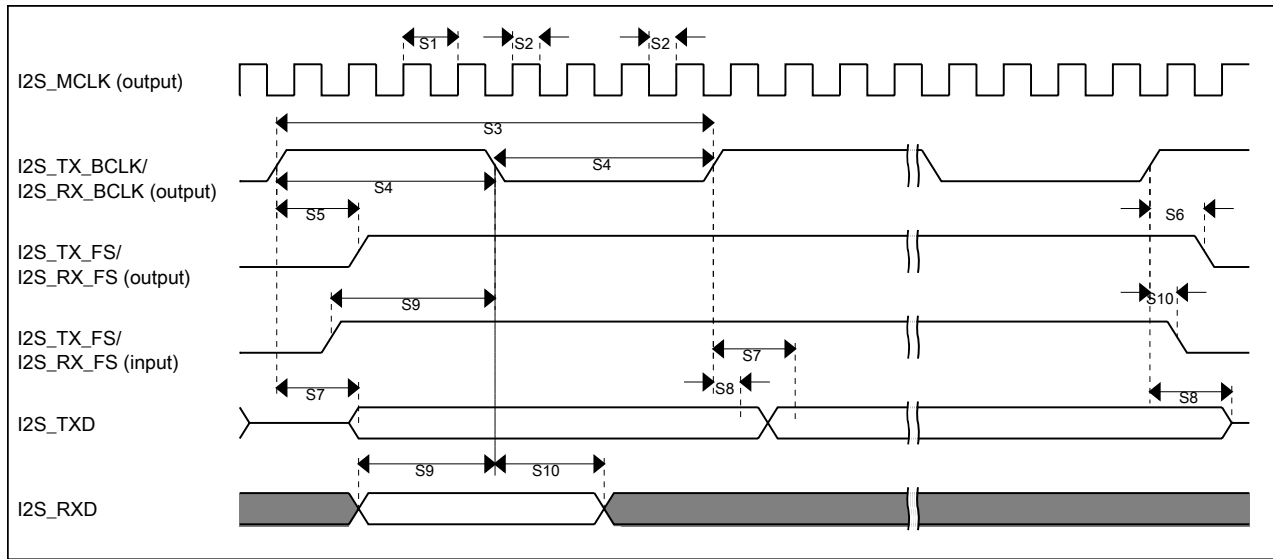
Figure 30. I2S/SAI timing — master modes
