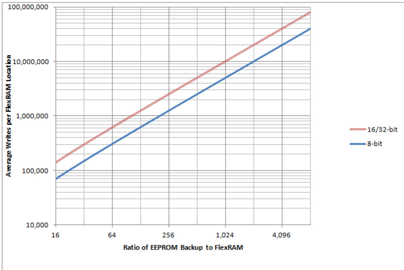
Figure 11. EEPROM backup writes to FlexRAM
