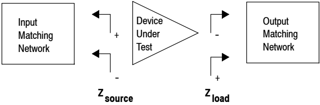
Figure 11. Series Equivalent Source and Load Impedance
