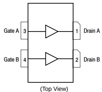
Figure 1. Pin Connections
