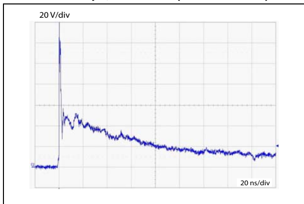
Figure 7. ESD response to ISO 10605, C = 150 pF, R = 330 Ω (+8 kV contact)
