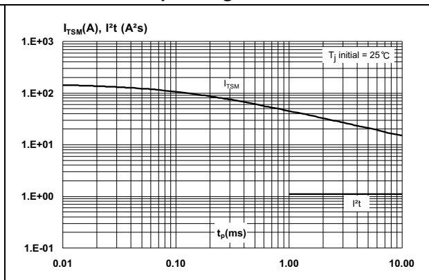
Figure 9. Non repetitive surge peak on-state current for a sinusoidal pulse, and corresponding value of I^2t
