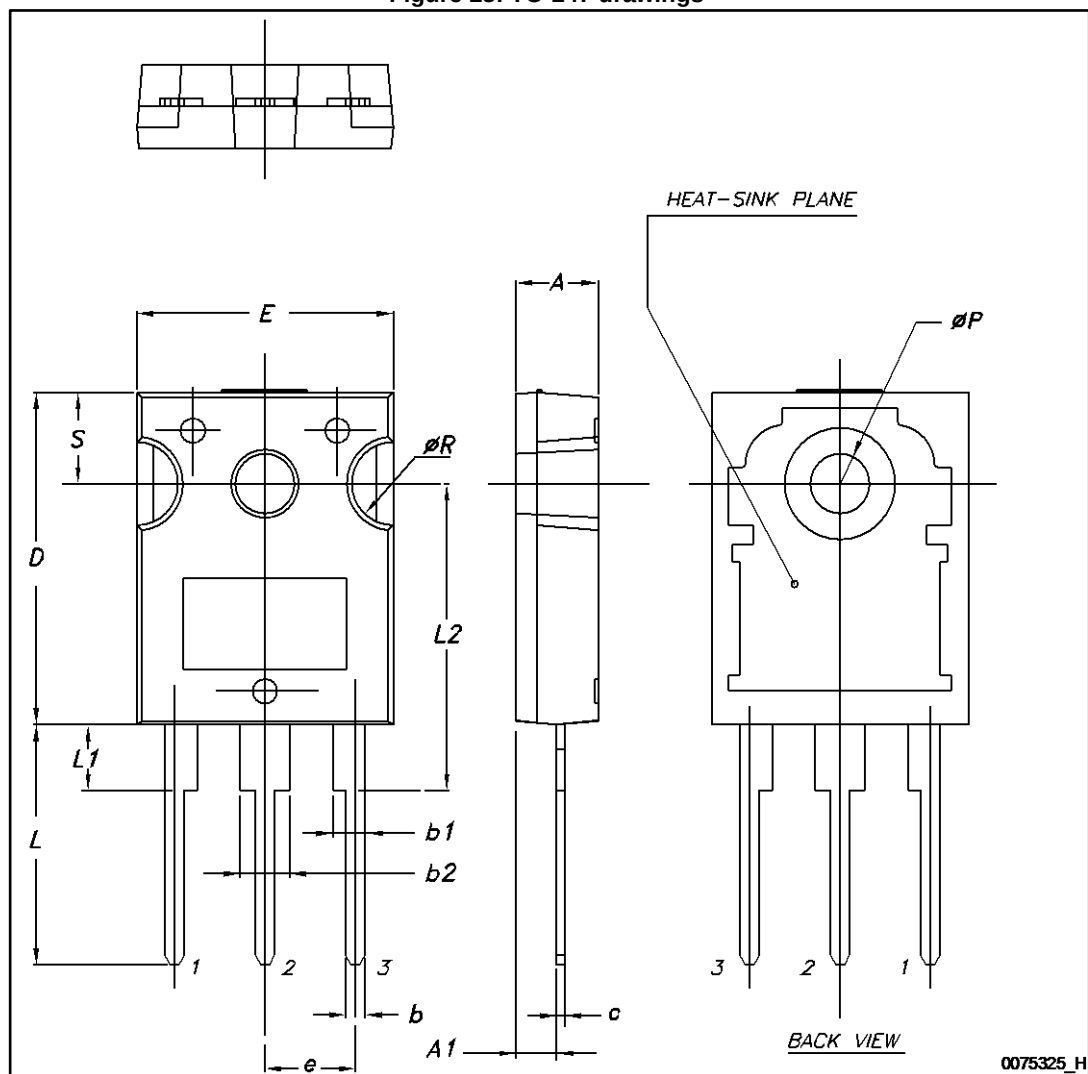
Figure 25: TO-247 drawings
