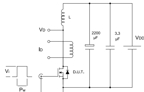
Figure 21: Unclamped inductive load test circuit
