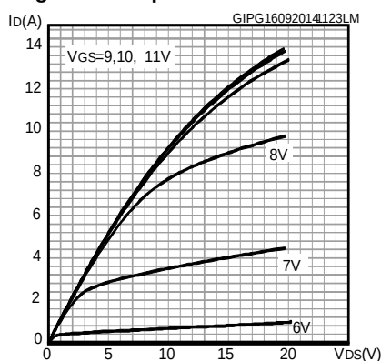
Figure 8: Output characteristics
