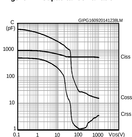
Figure 12: Capacitance variation
