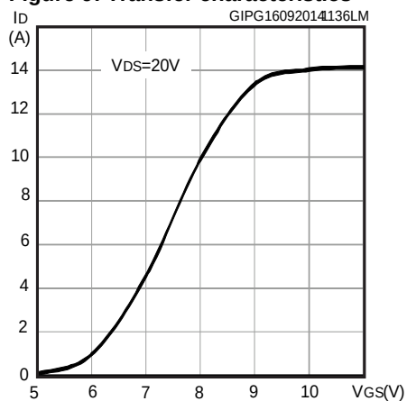
Figure 9: Transfer characteristics
