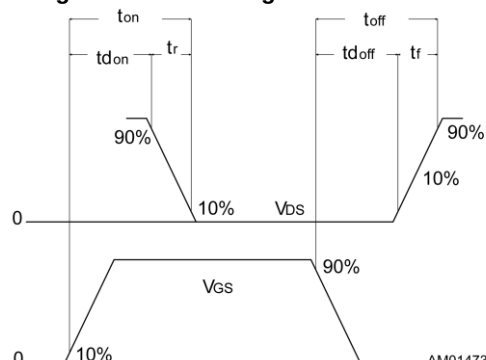
Figure 23: Switching time waveform
