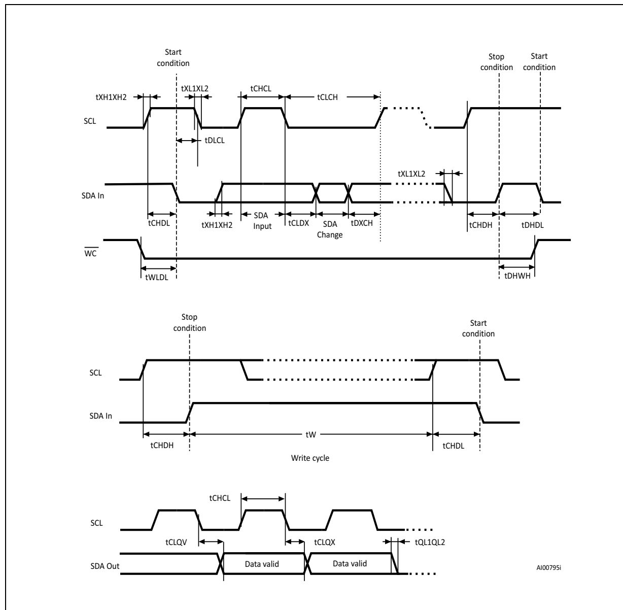
Figure 12. AC waveforms
