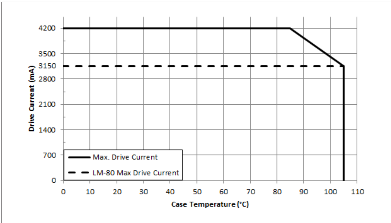
Figure 2: Vero 29 Drive Current Derating Curve
