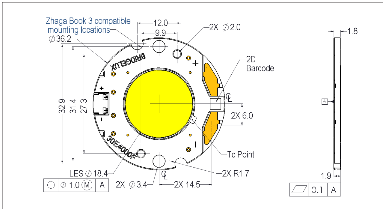
Figure 22: Drawing for Vero 18 LED Array
