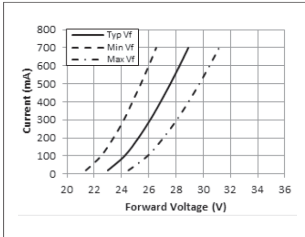
Figure 3: Vero 10 Drive Current vs. Forward Voltage ( T_j=T_c=25^\circ\text{C} )
