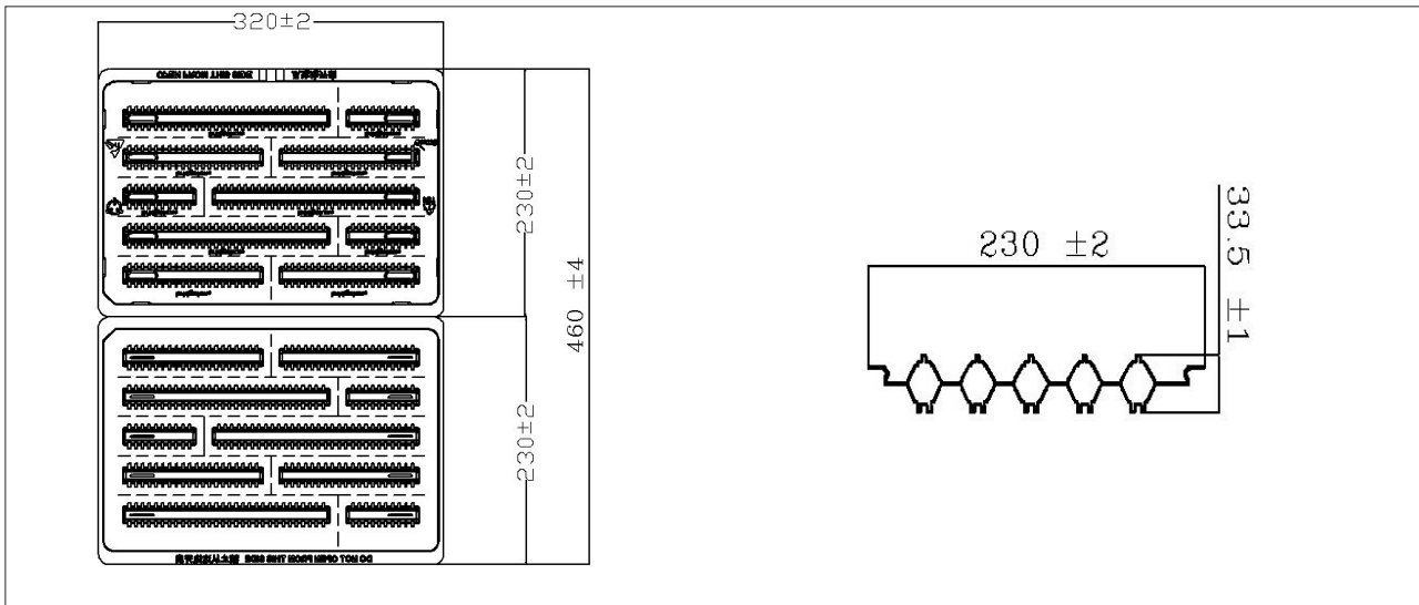
Figure 24: Drawing for Vero 10 Packaging Tray
