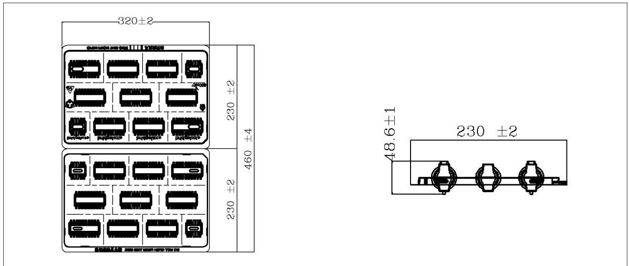
Figure 26: Drawing for Vero 18 Packaging Tray
