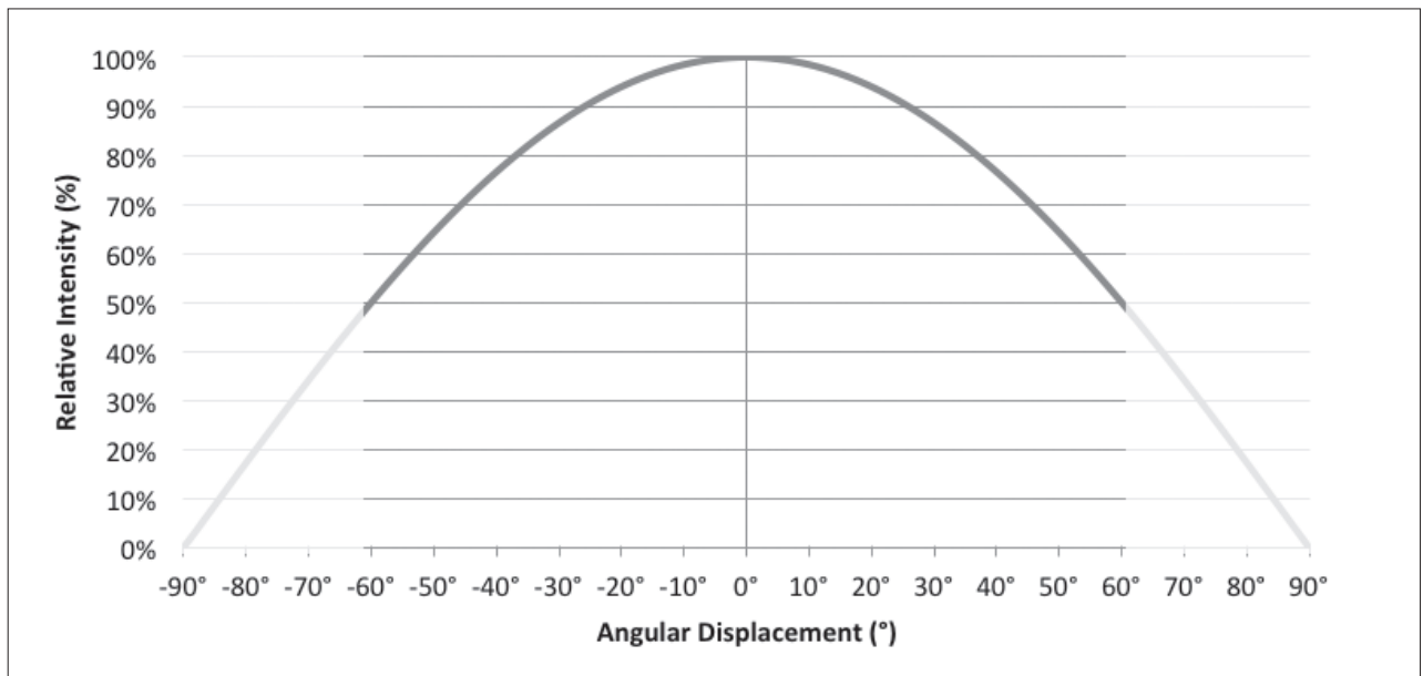
Figure 18: Typical Spatial Radiation Pattern
