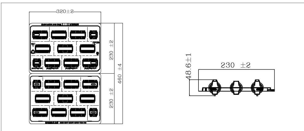
Figure 25: Drawing for Vero 13 Packaging Tray
