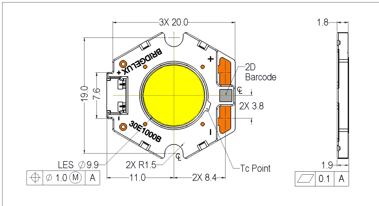
Figure 20: Drawing for Vero 10 LED Array
