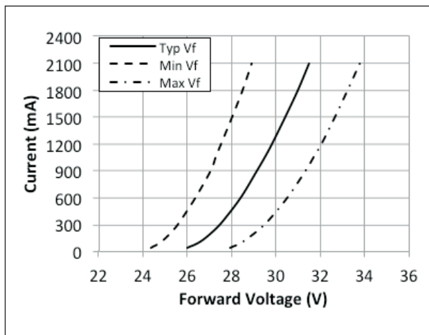
Figure 5: Vero 18 Drive Current vs. Forward Voltage ( T_j=T_c=25^\circ\text{C} )
